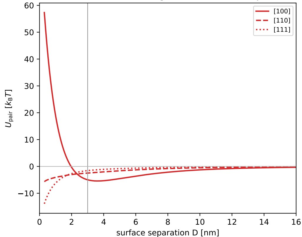
16 nm, centre line along [100]/[110]/[111], plan 3
