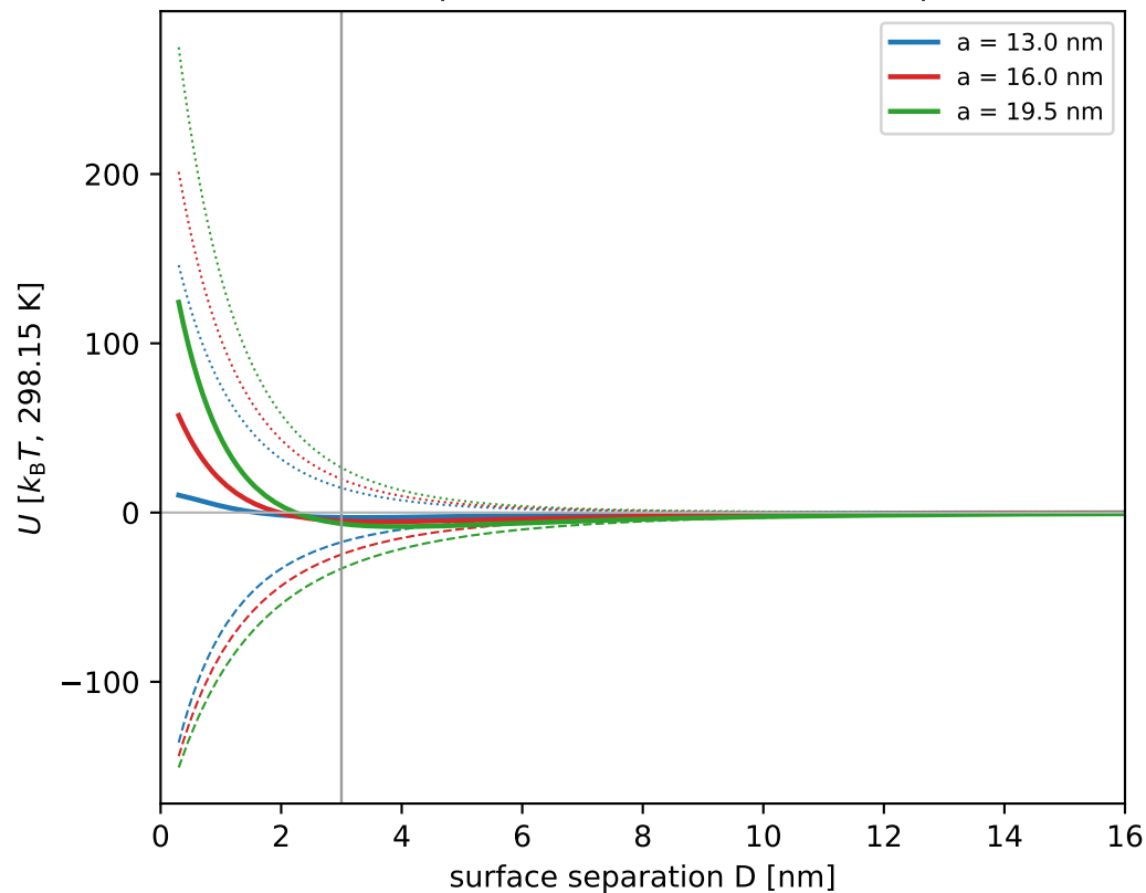
Face-to-face [100], singh_calibrated_si_mesh, transfer plan 3 (solid pair, dashed attr, dotted rep)
