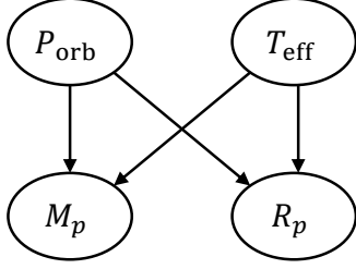
Figure 4. Preferred hot-Jupiter causal graph from BOSS with the FFML score. The inflation-relevant result is that R_p has direct parents P_{\text{orb}} and T_{\text{eff}} , but no direct M_p \rightarrow R_p edge after conditioning.
