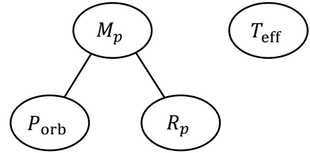
Figure 3. The causal structure found from super-Earth data using BOSS with FFML score. An undirected edge A - B suggests both directions are possible (either A \rightarrow B or A \leftarrow B ), as long as no new colliders are created. Here, the graph means that P \rightarrow M_p \rightarrow R_p , P \leftarrow M_p \leftarrow R_p , or P \leftarrow M_p \rightarrow R_p (but not P \rightarrow M_p \leftarrow R_p ), plus an isolated node T_{\star} , are equally possible statistically and are together the most likely causal structure.
