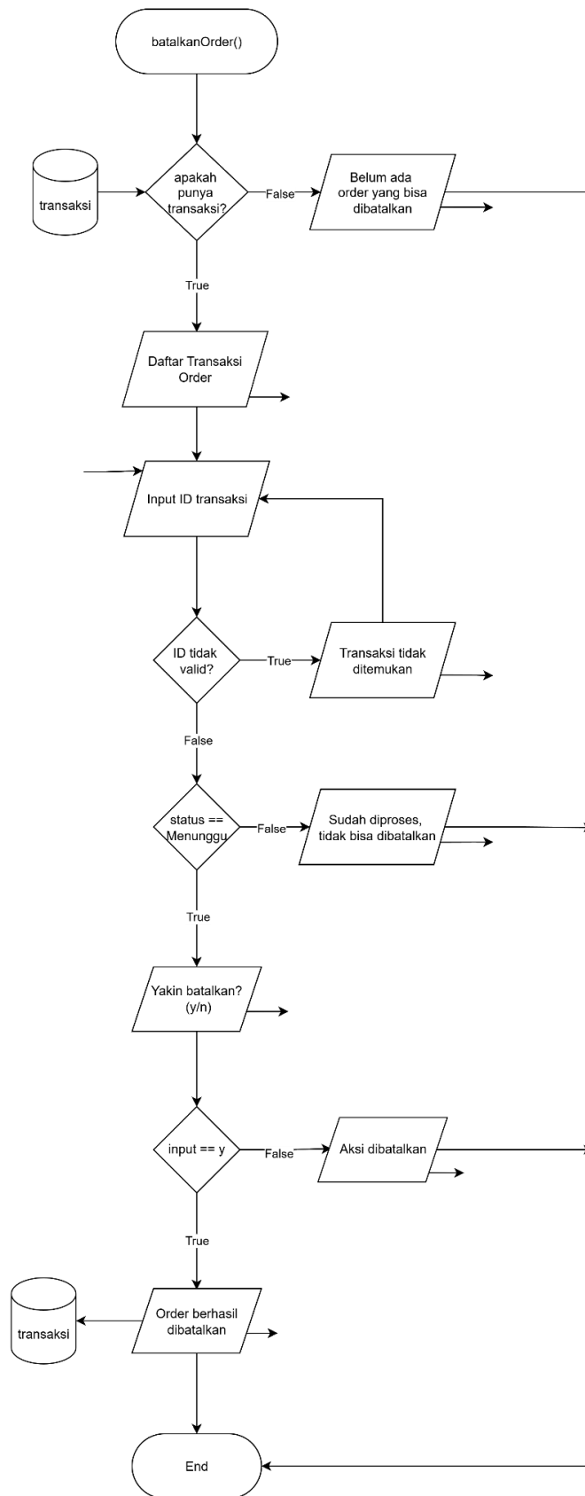
Gambar 2.1 Flowchart Fungsi Batalan Order
