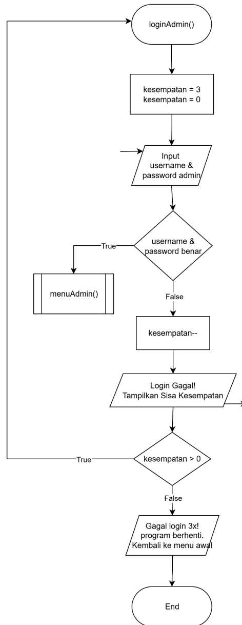
Gambar 2.2 Flowchart Fungsi Login Admin
