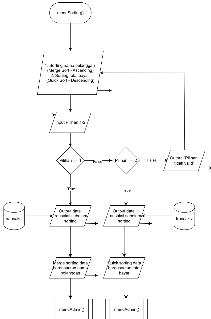
Gambar 2.15 Flowchart Fungsi Menu Sorting
