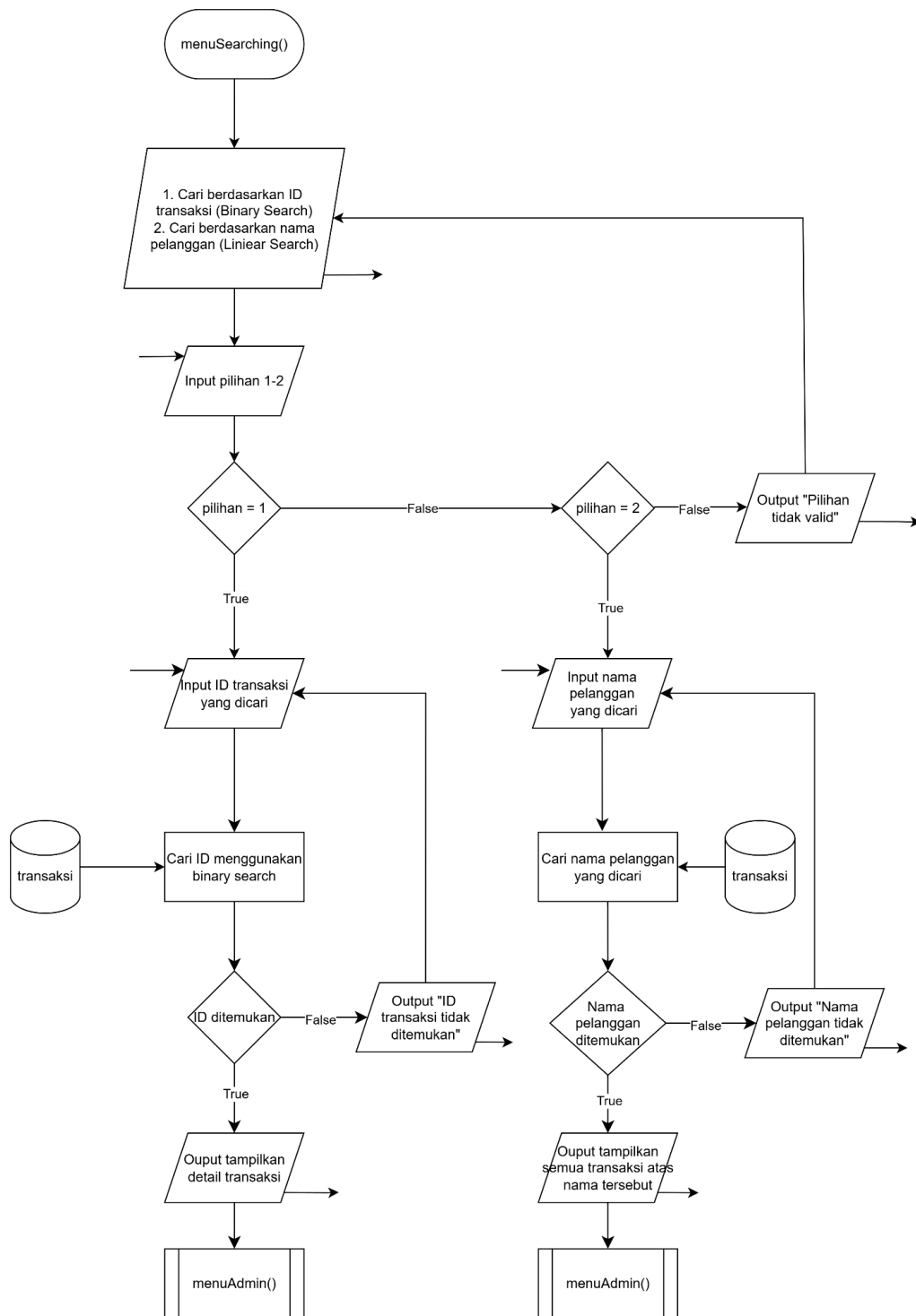
Gambar 2.16 Flowchart Fungsi Menu Searching
