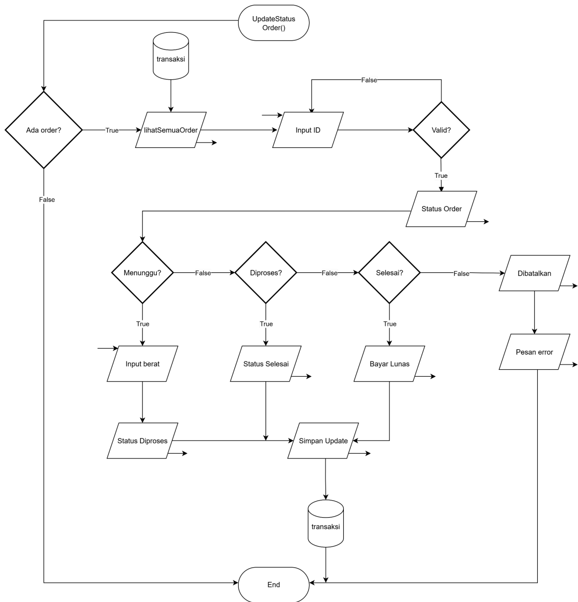
Gambar 2.13 Flowchart Fungsi Update Status Order
