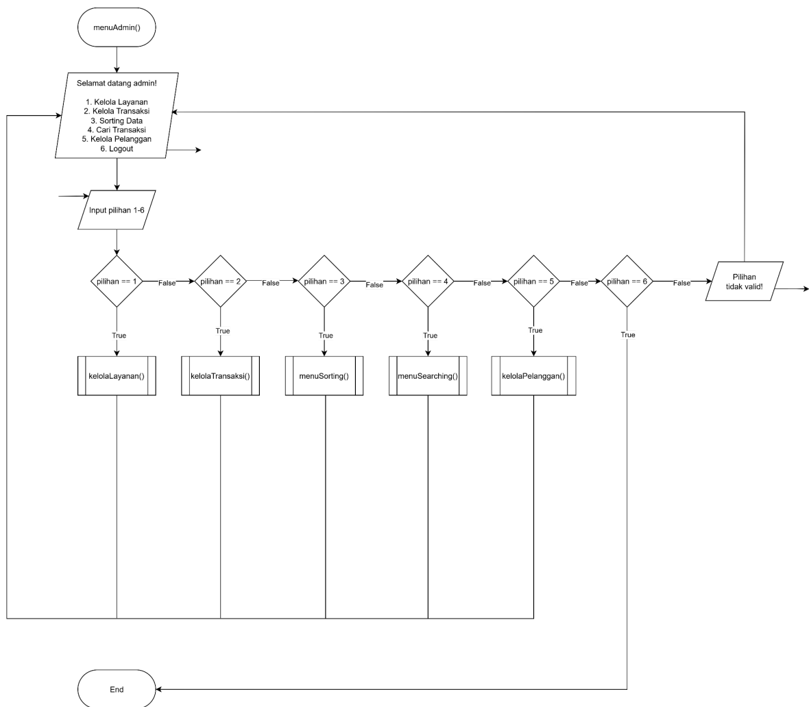
Gambar 2.5 Flowchart Menu Admin
