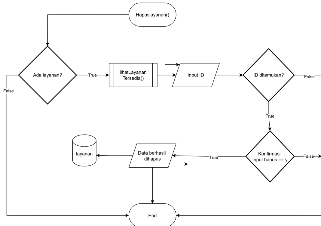
Gambar 2.10 Flowchart Fungsi Hapus Layanan
