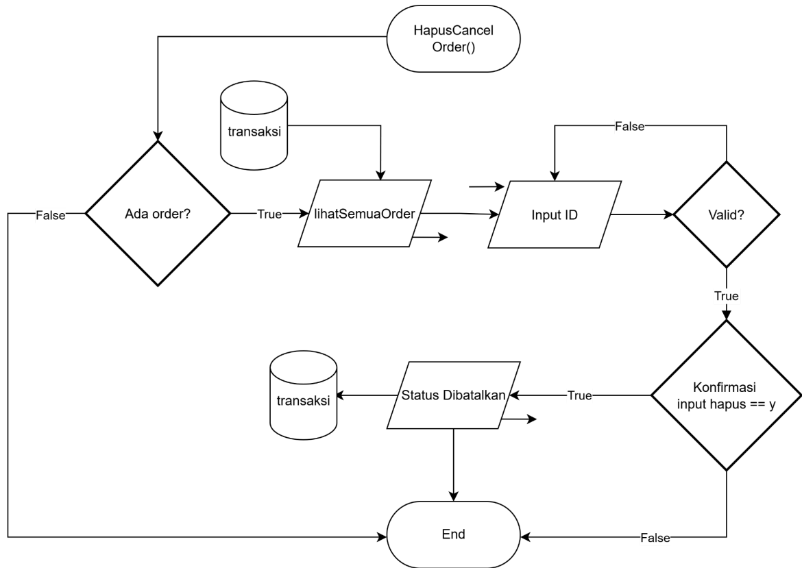
Gambar 2.14 Flowchart Fungsi Hapus Cancel Order
