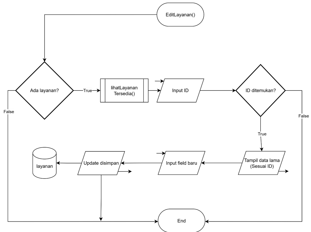
Gambar 2.9 Flowchart Fungsi Edit Layanan
