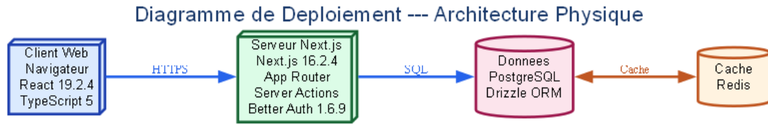
FIGURE 10 – Diagramme de Deploiement — Architecture Physique de SaaS Directory
