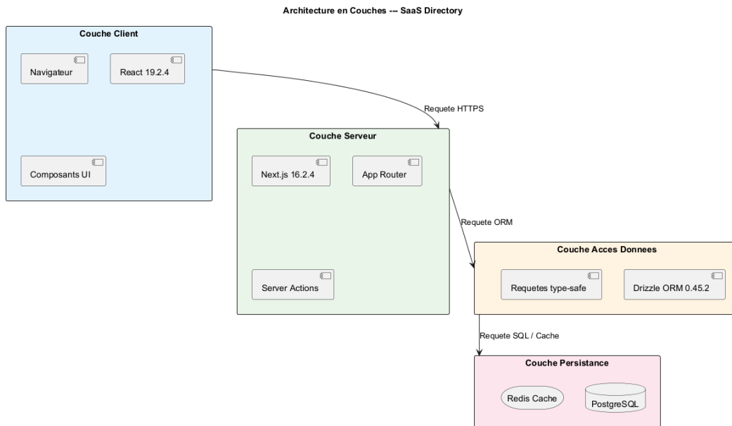
FIGURE 1 – Architecture en Couches — SaaS Directory
