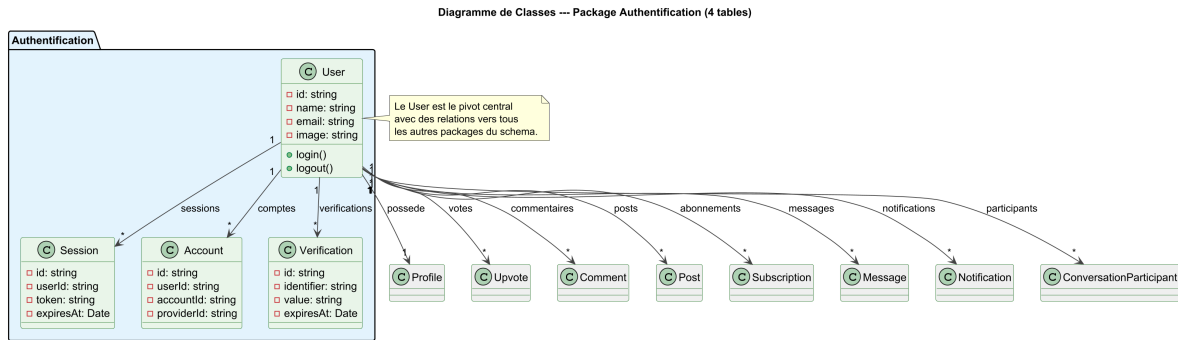
FIGURE 5 – Diagramme de Classes — Package Authentication (4 tables)
