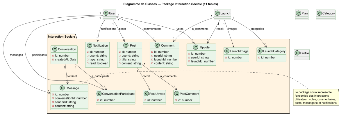
FIGURE 7 – Diagramme de Classes — Package Interaction Sociale (11 tables)
