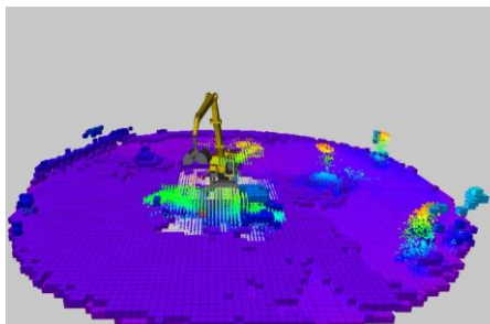
A. Large-scale material handling
