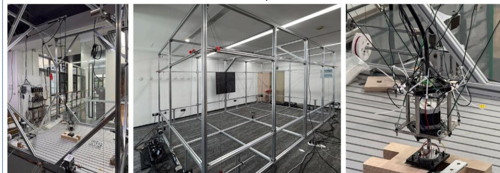
F. MR-guided cable-robot assembly
