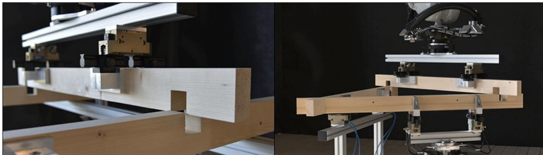
A. Timber-joint insertion
