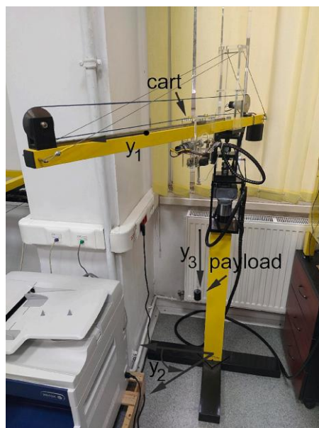
A. Laboratory tower-crane safe control
