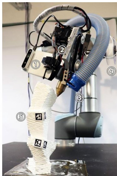
A. Robotic additive manufacturing
