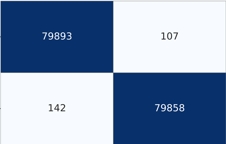
Hybrid Fusion (0.7 ML + 0.3 Rule)
