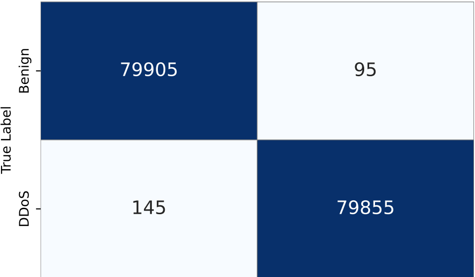
ML-Only (Random Forest)
