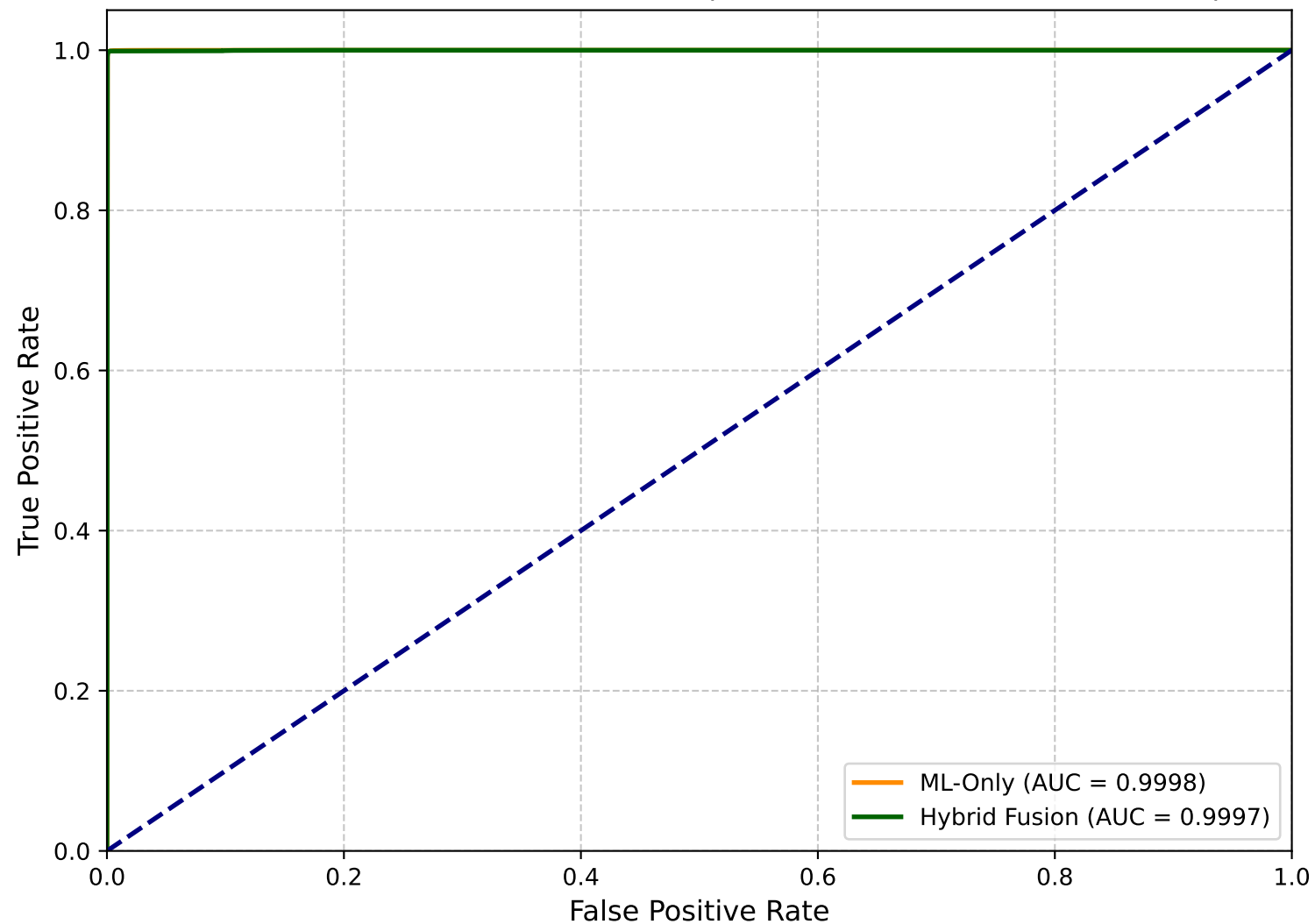
ROC Curves - Offline Evaluation (CICIDS2019 Balanced Test Set)
