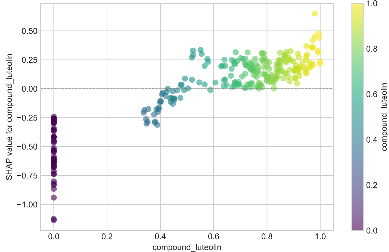
SHAP Dependence: compound_luteolin → Root Length Mm
