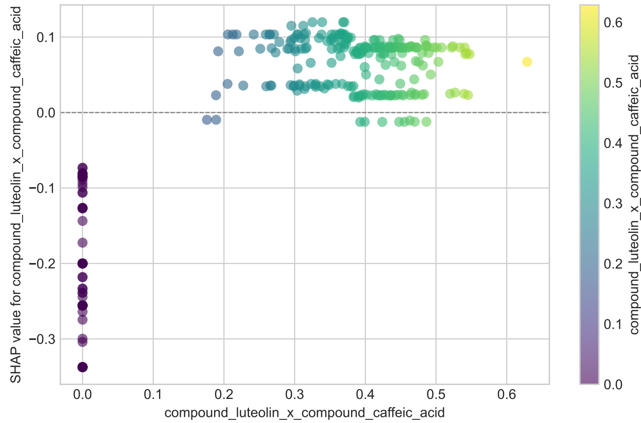
SHAP Dependence: compound_luteolin_x_compound_caffeic_acid → Germination Percent
