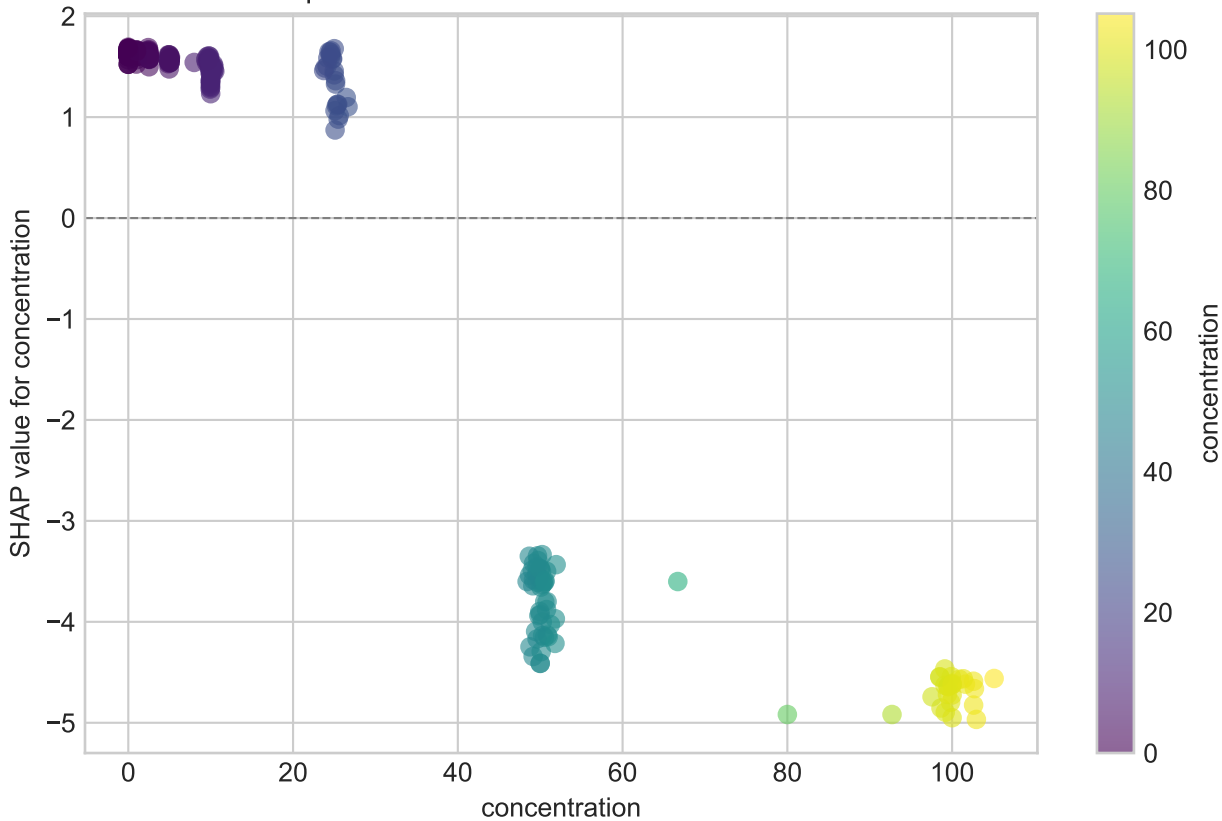
SHAP Dependence: concentration → Germination Percent
