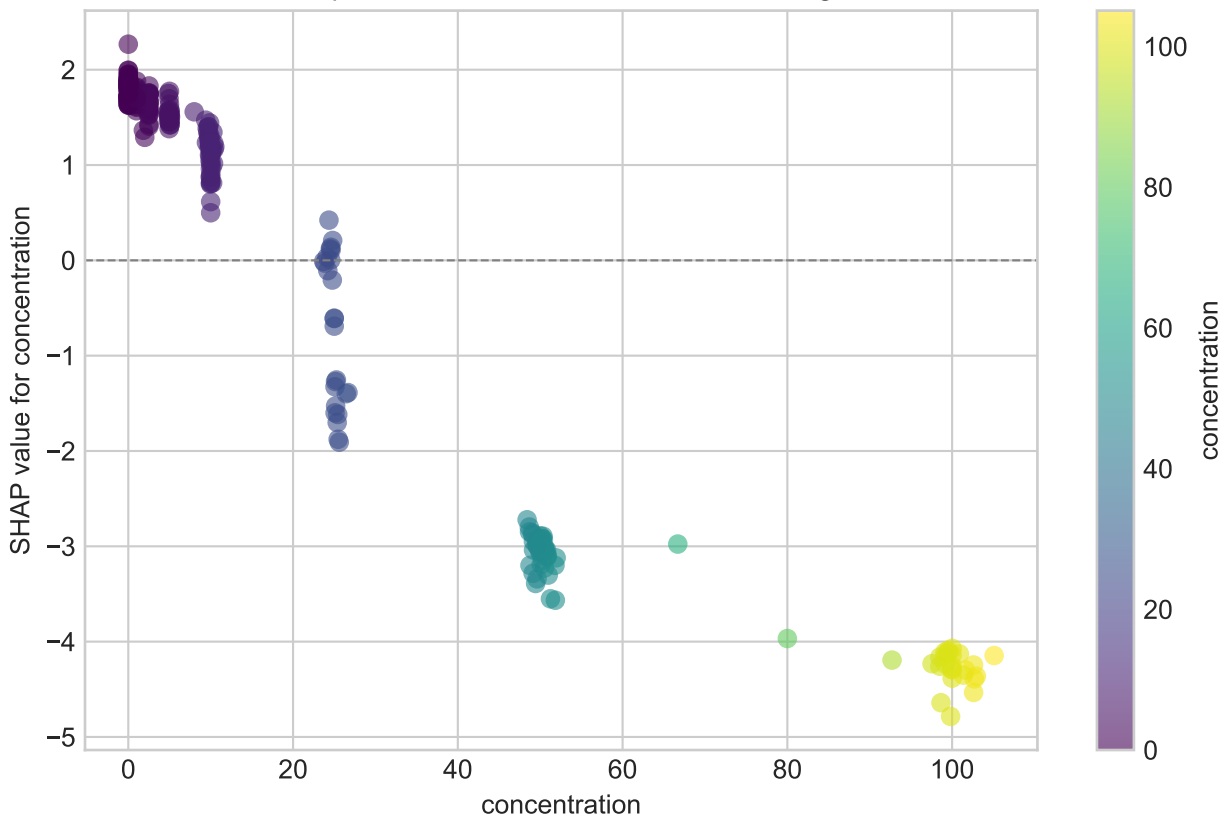
SHAP Dependence: concentration → Root Length Mm
