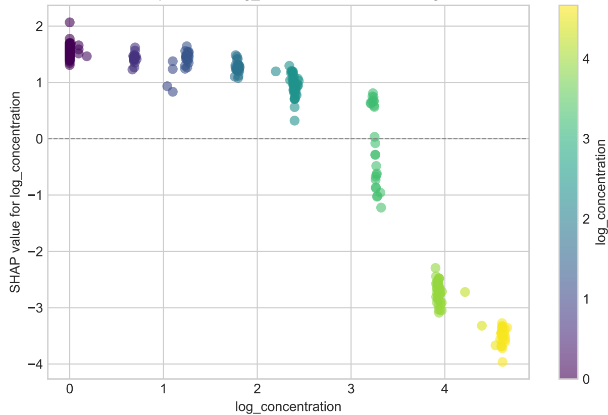
SHAP Dependence: log_concentration → Root Length Mm
