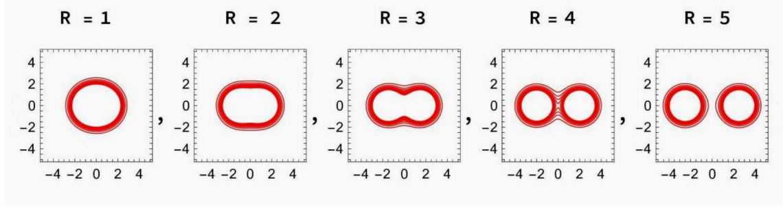
Figure 3.2: Gerade orbitals obtained from the LCAO approximation. The graph shows the overlap of the electronic orbitals for different values of the internuclear distance R
