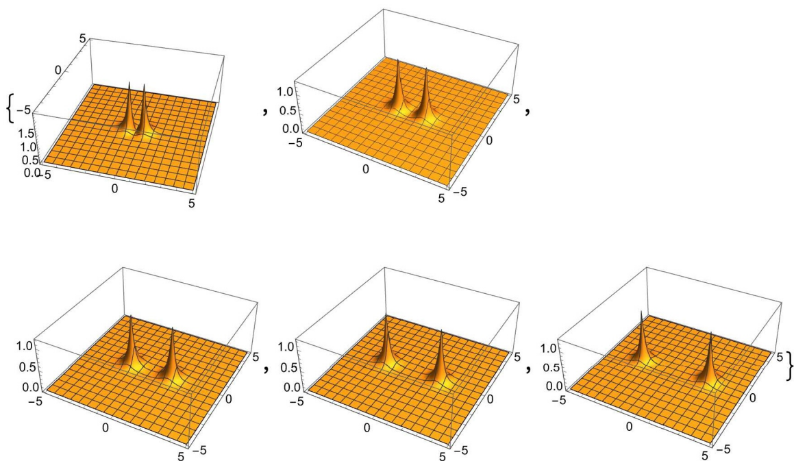
Figure 3.5: Ungerade orbitals in 3D from the same LCAO approximation. The graph shows the magnitude of the potential function for different values of the internuclear distance R
