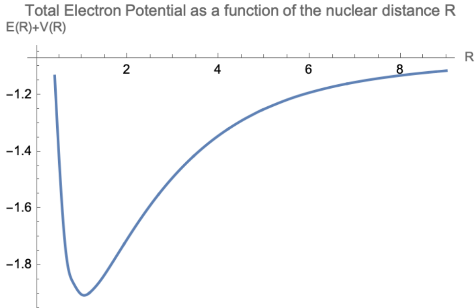
Figure 3.8: Total electron potential energy as function of internuclear distance R for 3D H_2^+ , given as E(R) + V(R)
