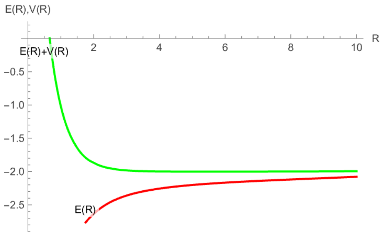
Figure 4.3: H_2^+ energy and potential curves for the 1s_u^+ state
