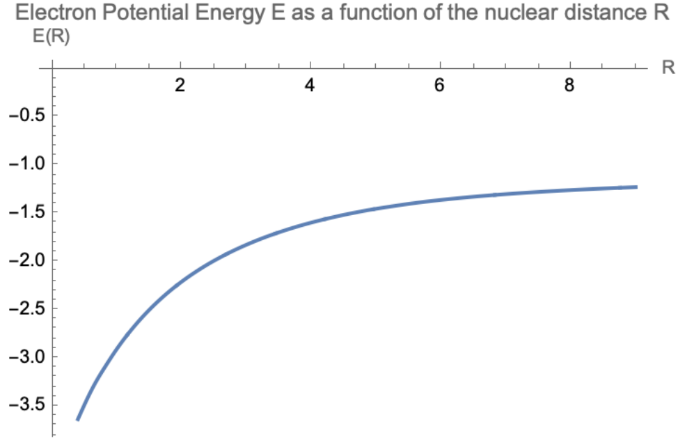
Figure 3.7: Electron potential energy as function of internuclear distance R for 3D H_2^+
