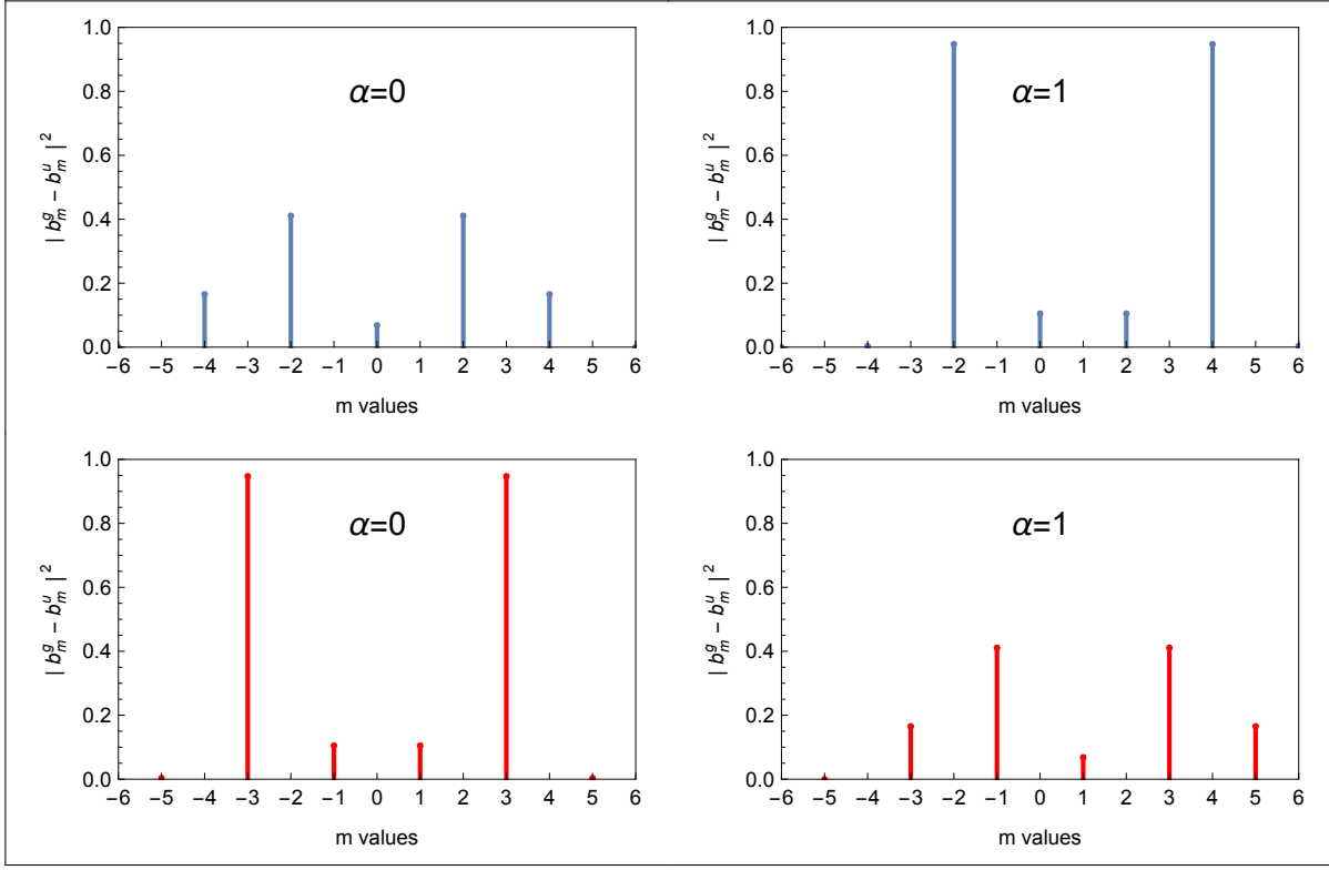
Figure 5.2: Collision temperature T = 10 K. Blue icons refer to a bosonic base, and red icons to a fermionic base.
