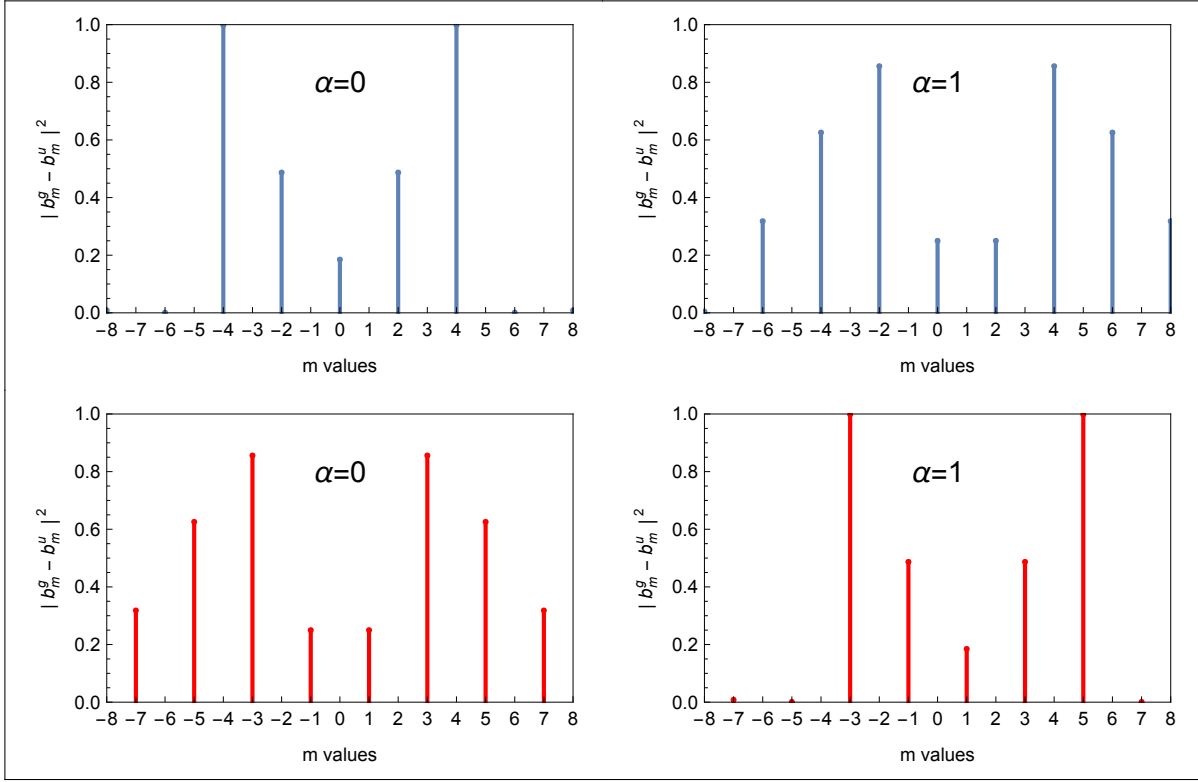
Figure 5.4: Collision temperature T = 100 K . Blue icons refer to a bosonic base, and red icons to a fermionic base.
