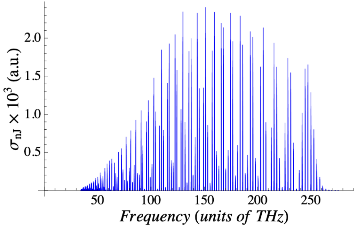
Figure 1.2: Emission spectrum for the radiative association process at a gas temperature of 1mK.
