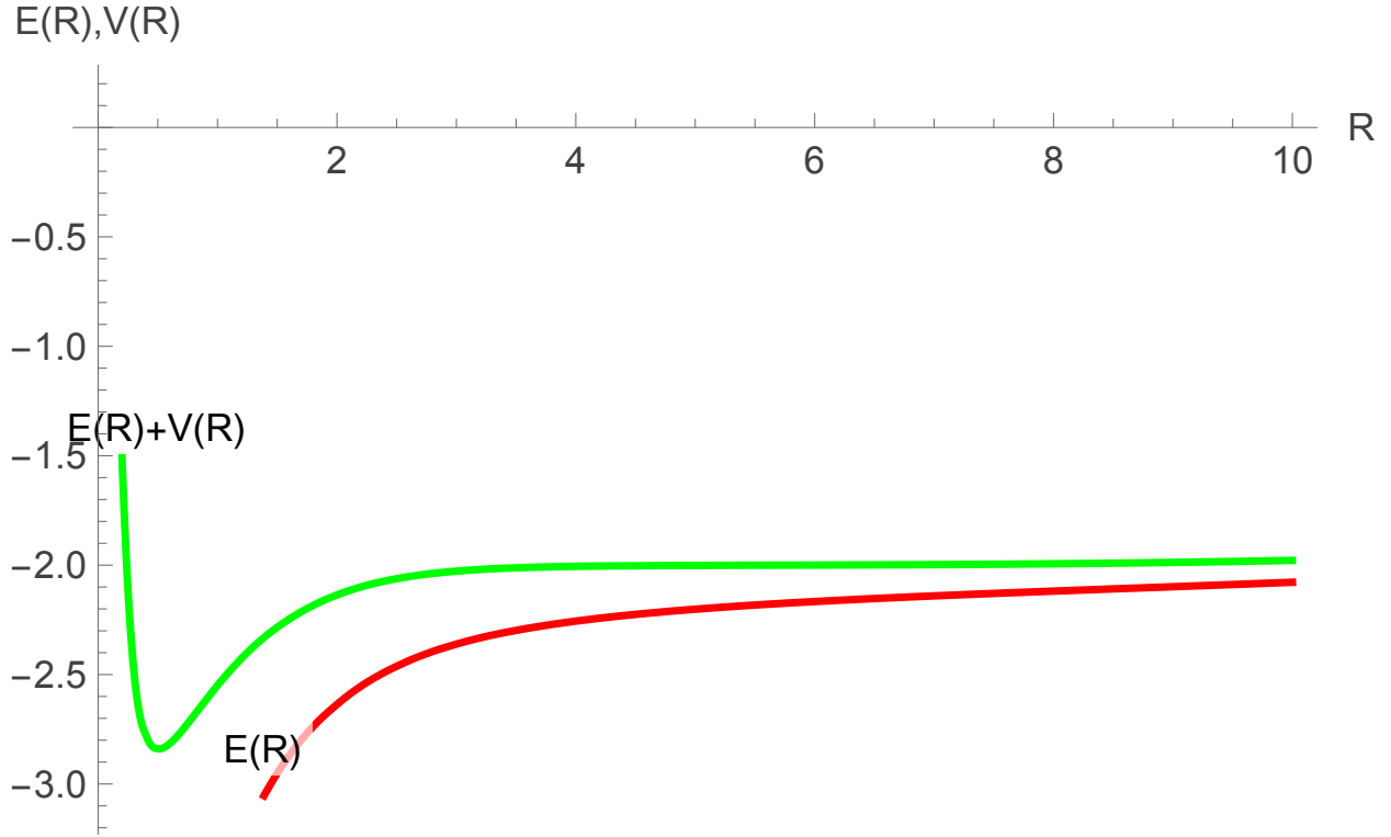
Figure 4.2: H_2^+ energy and potential curves for the 1s_g^+ state
