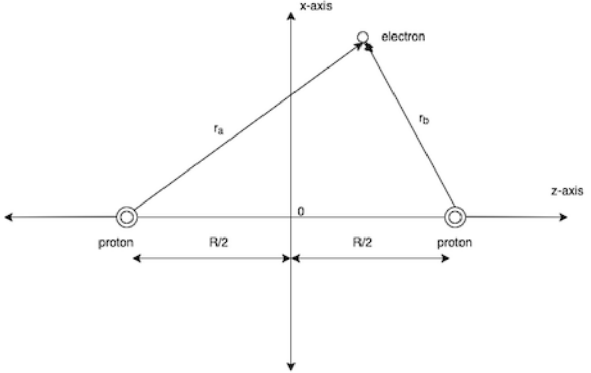
Figure 3.6: H_2^+ ion, showing the position of the nuclei at distance R , and a coordinates of an electron
