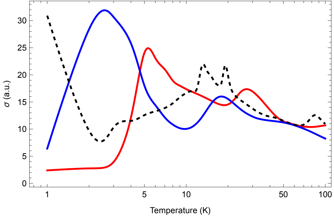
Figure 5.6: Total RCT cross sections. Solid lines refer to \alpha = 0 (i.e., absence of flux tube), for the bosonic base (blue line) and the fermionic base (red line) respectively. The dashed line refers to a semion ( \alpha = 1/2 ), and the cross section is identical for both fermionic and bosonic bases.
