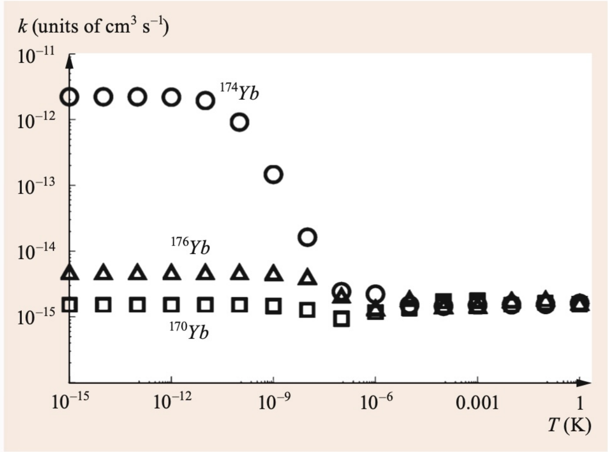
Figure 1.3: Isotopic dependence of radiative association into the \text{YbCa}^+ molecular ion
