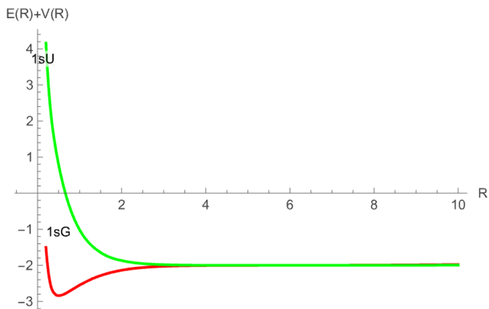
Figure 4.4: H_2^+ potential curves for the first gerade (red) and first ungerade (green) states
