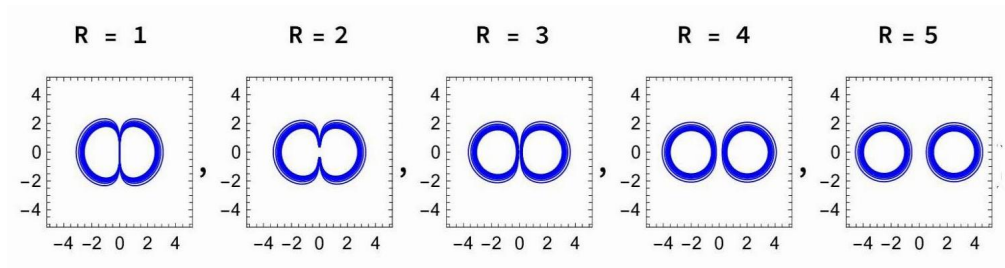
Figure 3.4: Ungerade orbitals obtained from the LCAO approximation. The graph shows the overlap of the electronic orbitals for different values of the internuclear distance R
