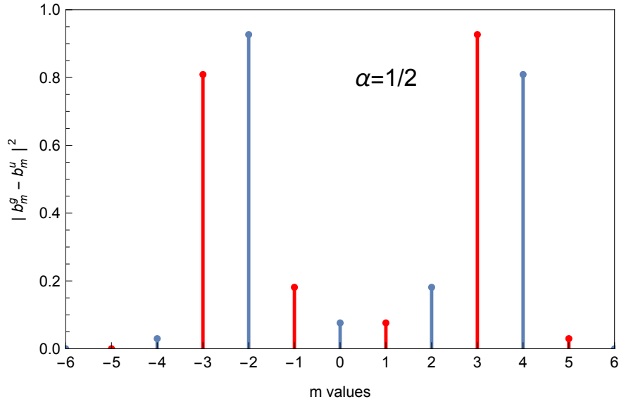
Figure 5.3: Collision temperature T = 10 K. Blue icons refer to a bosonic base, and red icons to a fermionic base.
