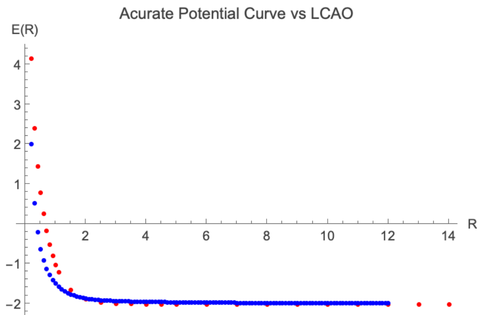
Figure 3.1: Accurate potential curve (red) vs LCAO approximation (blue) for the H_2^+ 1st excited ungerade state
