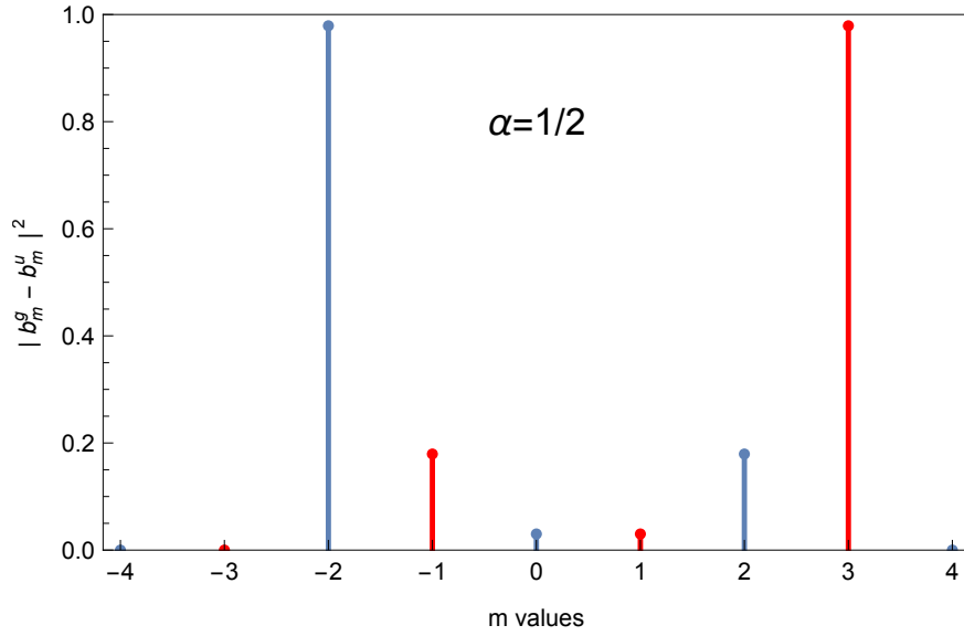
Figure 6.3: Collision temperature T = 1\text{ K} . Blue icons refer to a bosonic base, and red icons to a fermionic base.
