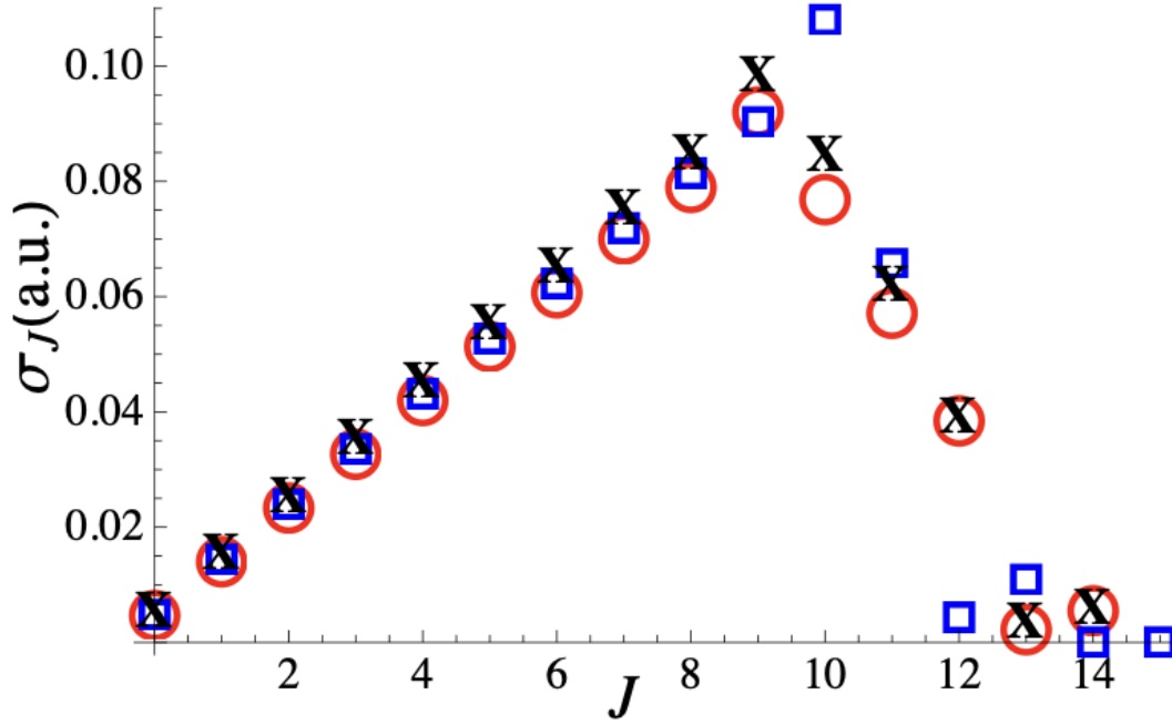
Figure 2.3: Plot of various cross sections as a function of incoming partial wave J . Circles represent data for the radiative association cross sections, Xs represent an upper bound for the total (association + radiative charge transfer), and squares represent the data for the total radiative relaxation obtained using the optical potential method.
