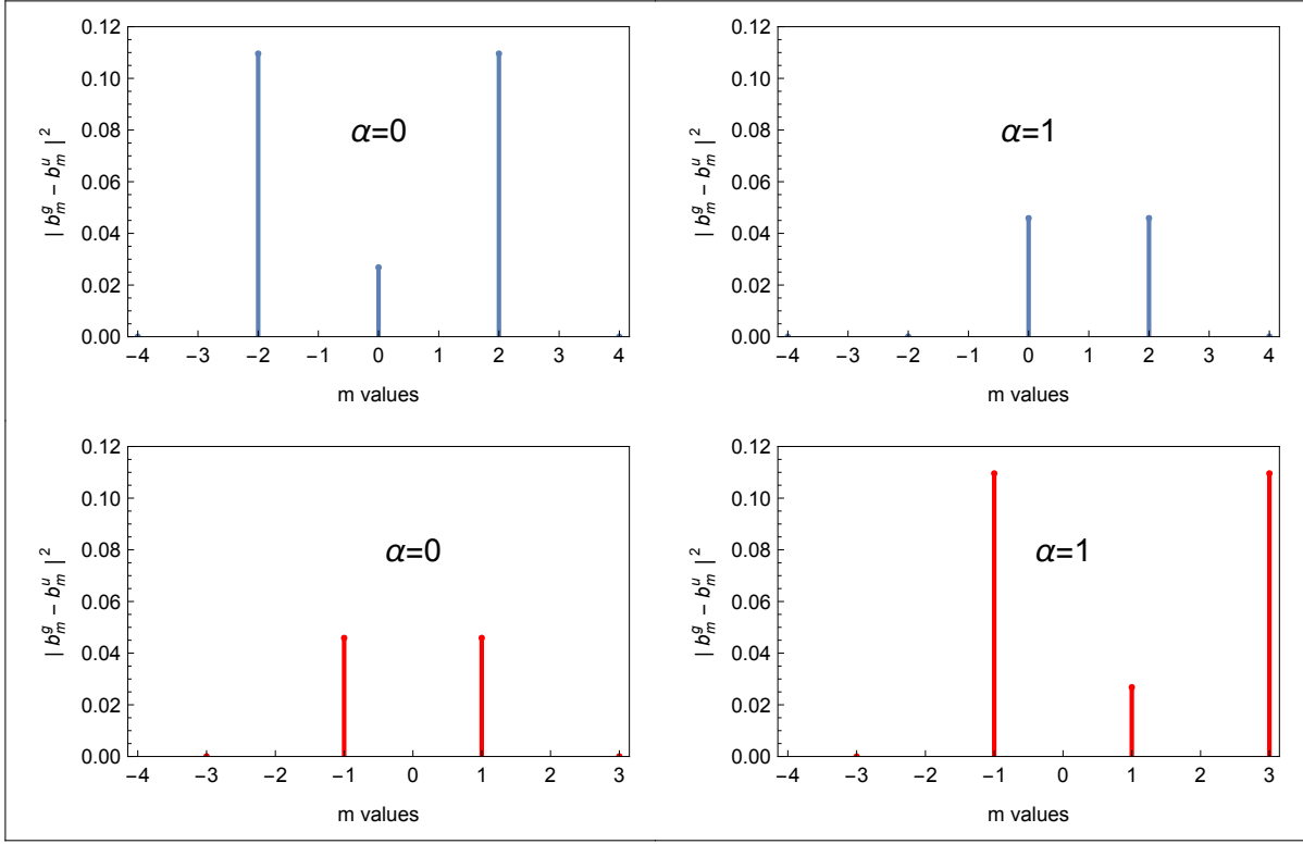
Figure 6.2: Collision temperature T = 1\text{ K} . Blue icons refer to a bosonic base, and red icons to a fermionic base.
