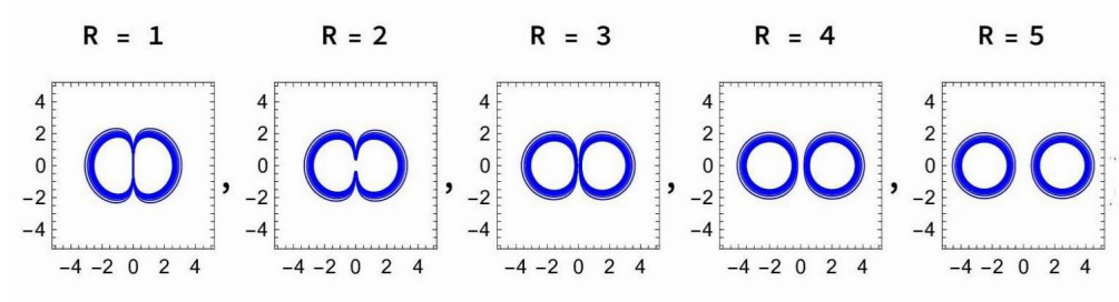
Figure 4.6: Ungrade orbitals obtained from the LCAO approximation. The graph shows the overlap of the electronic orbitals for different values of the internuclear distance R
