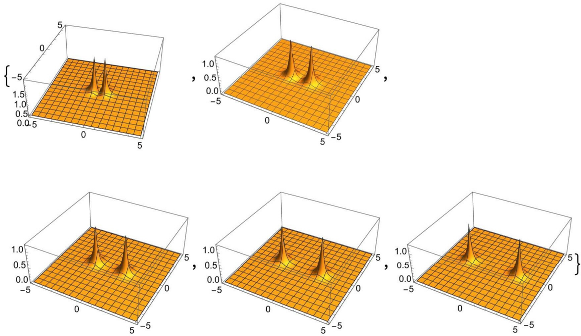
Figure 4.7: Ungrade orbitals in 3D from the same LCAO approximation. The graph shows the magnitude of the potential function for different values of the internuclear distance R
