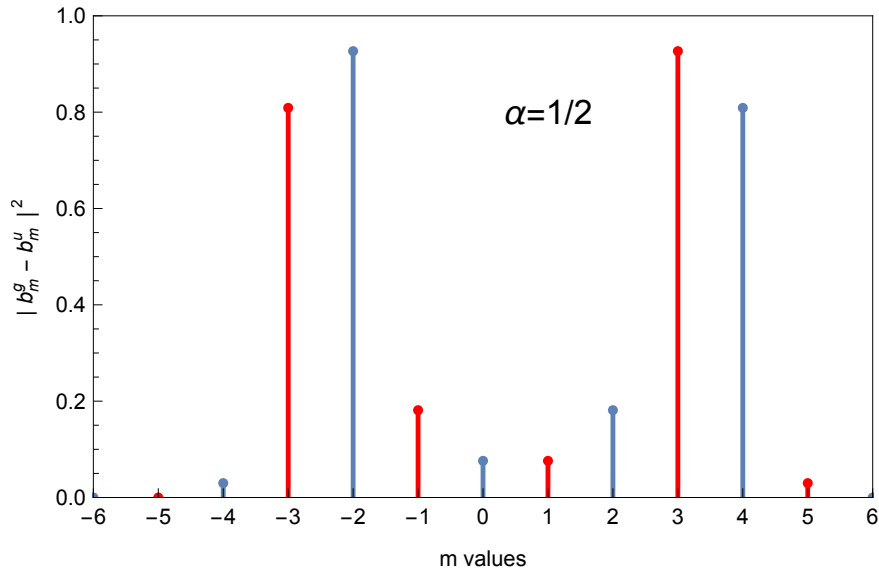
Figure 6.5: Collision temperature T = 10 K . Blue icons refer to a bosonic base, and red icons to a fermionic base.
