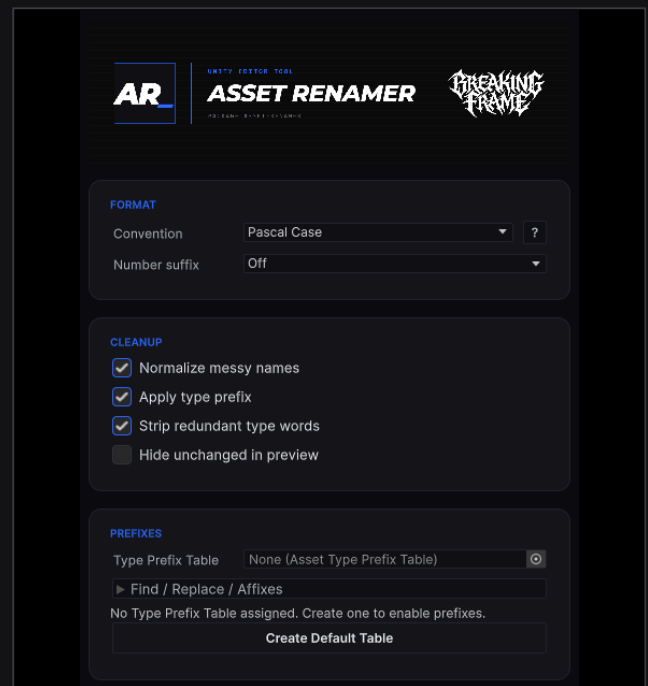
THE ASSET RENAMER EDITOR WINDOW ON FIRST OPEN.
