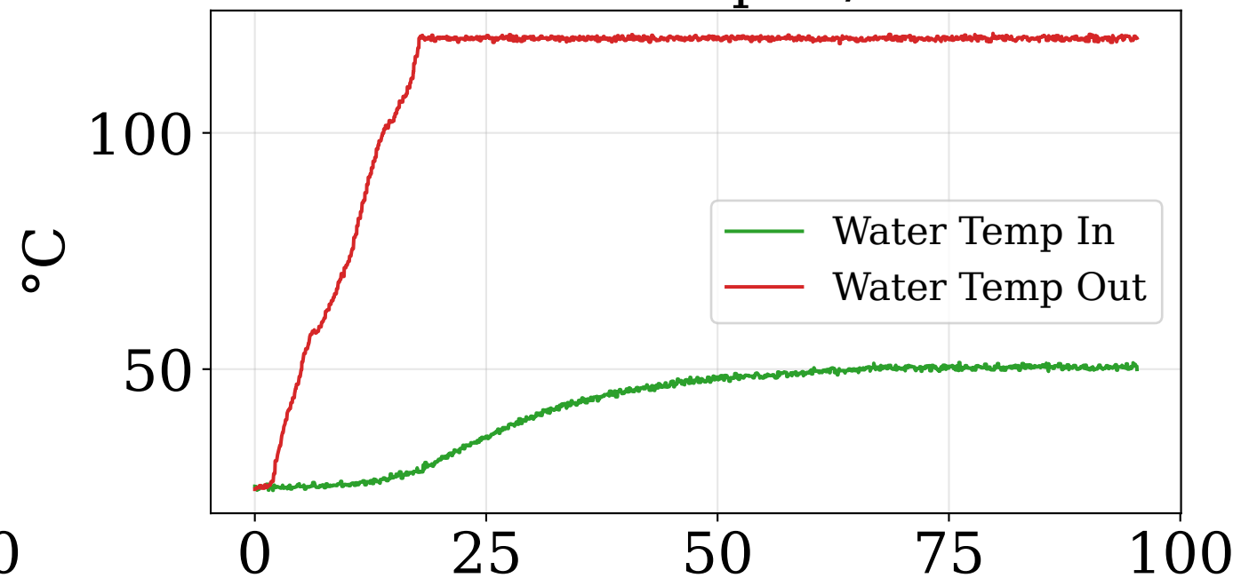
Water Temp In/Out
