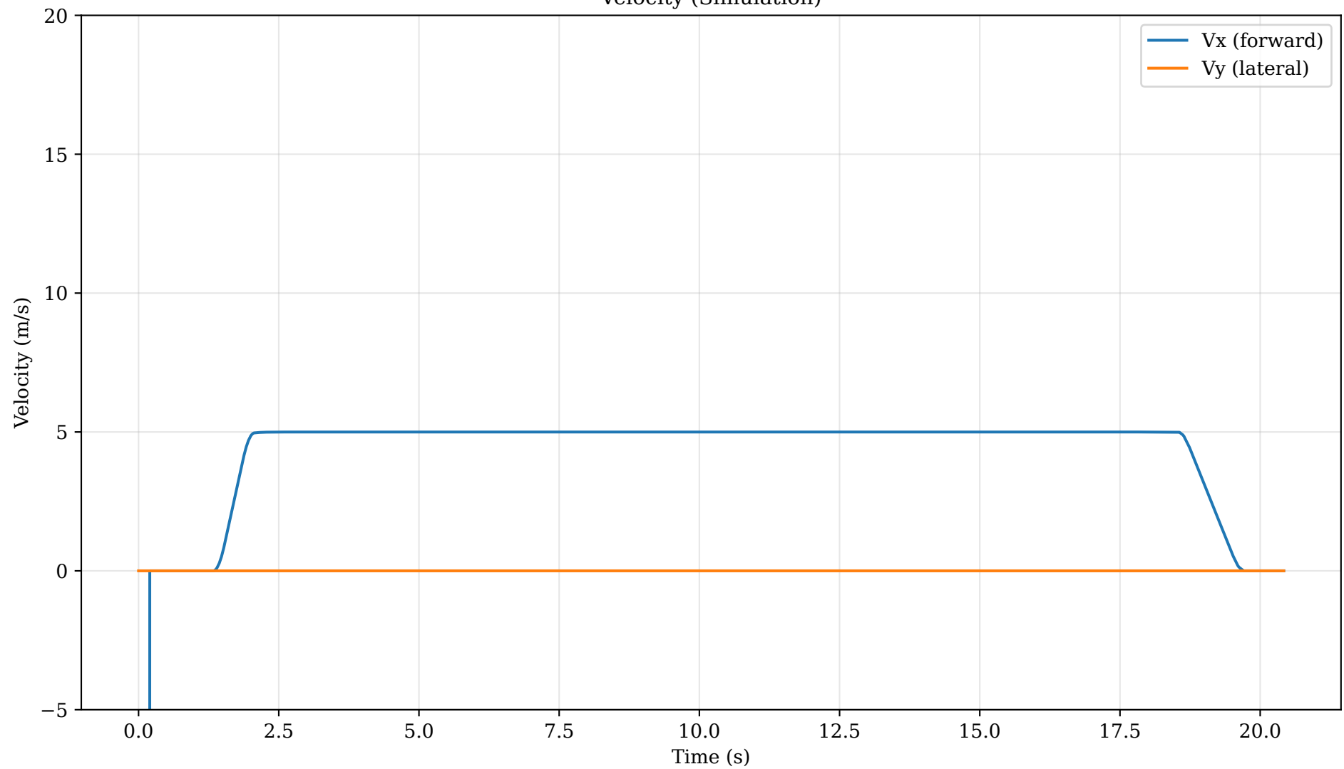
Velocity (Simulation)
