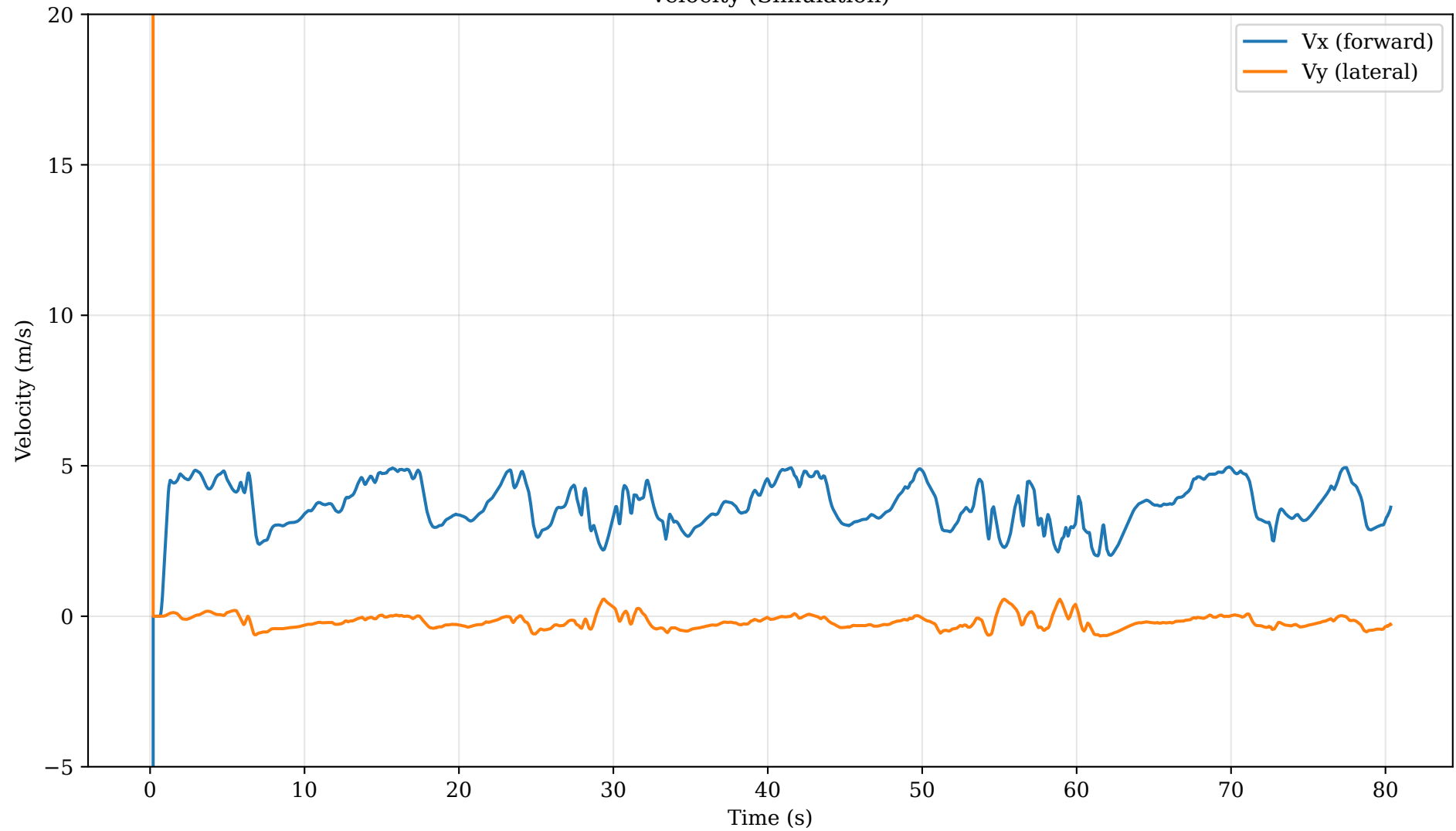
Velocity (Simulation)
