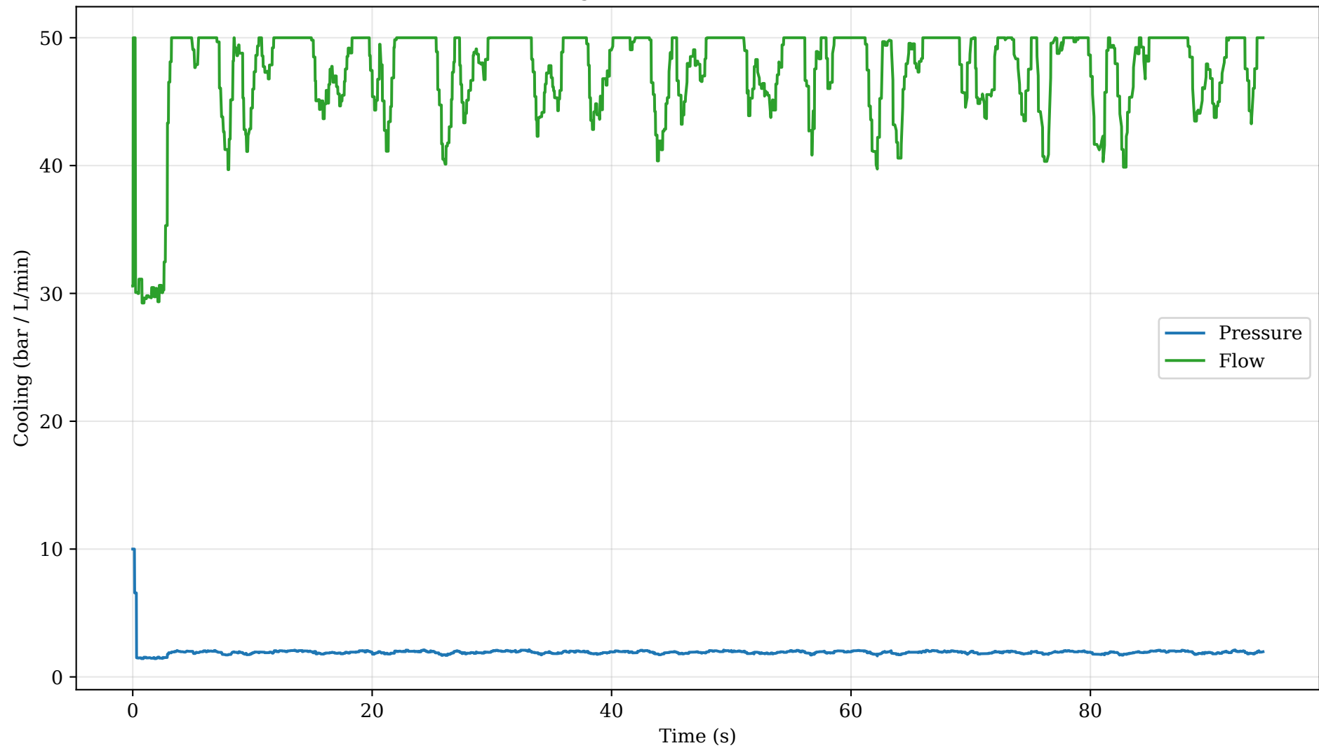
Cooling Pressure/Flow (Simulation)
