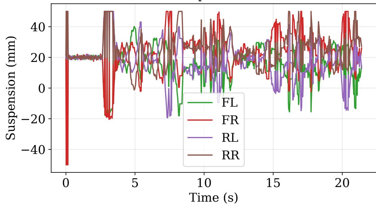
Suspensions
