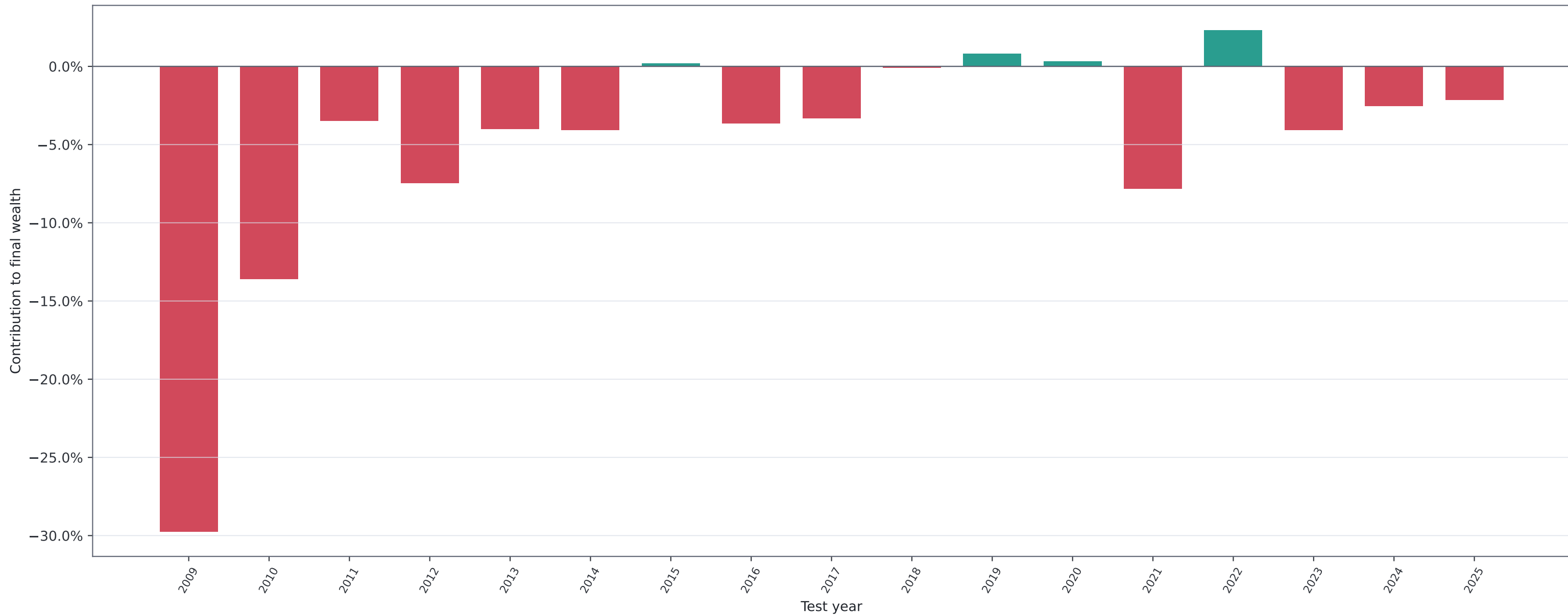
Fold-Level Cumulative Net Return Contribution (sum = -82.3%)
