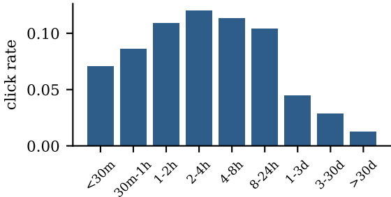
EB-NeRD test: click rate by article age
