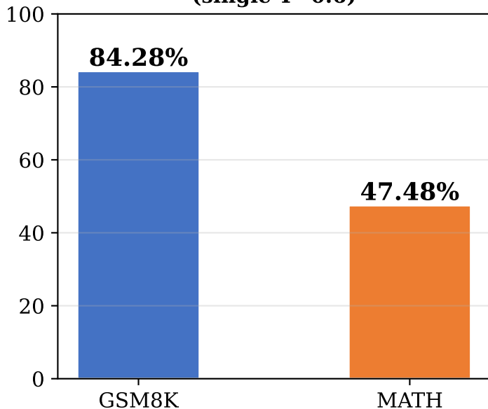
Teacher Total Accuracy (single T=0.6)
