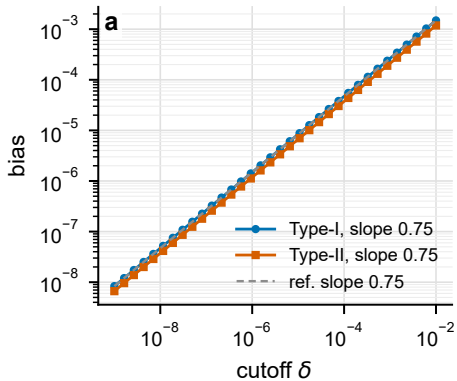
regularization bias, \alpha = 1.50
