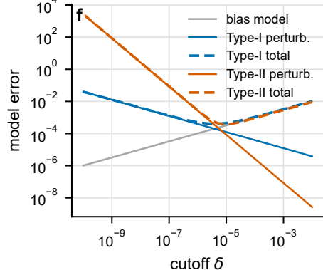
U-shaped trade-off, \alpha = 1.75
