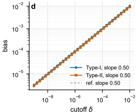
regularization bias, \alpha = 1.75
