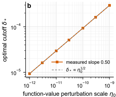
Type-II \eta_0 -dominated optimum
