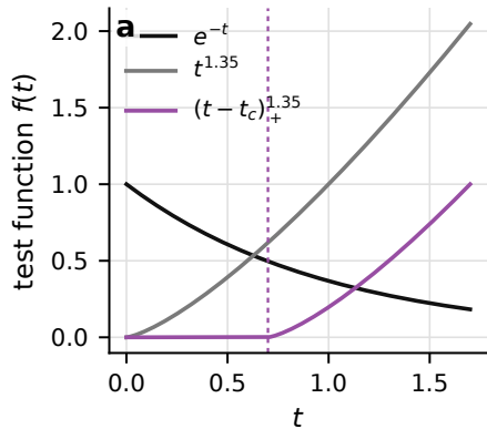
smooth vs non-smooth tests
