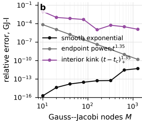
regularity controls convergence
