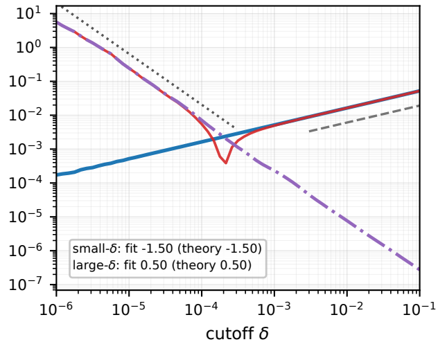
Type-II, \alpha = 1.50
