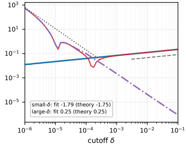
Type-II, \alpha = 1.75
