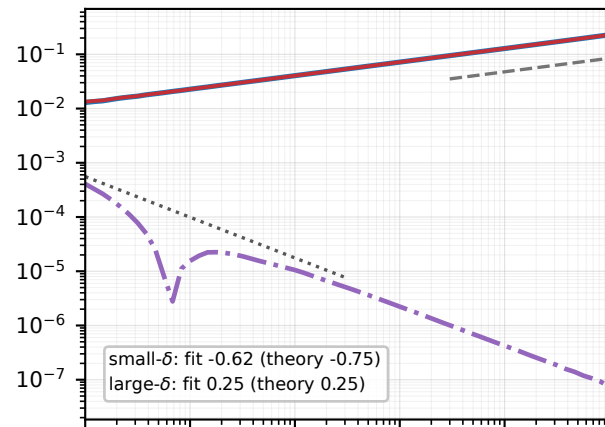
Type-II, \alpha = 1.75
