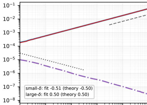
Type-II, \alpha = 1.50
