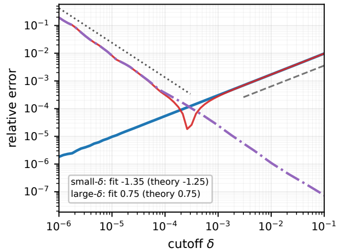
Type-II, \alpha = 1.25
