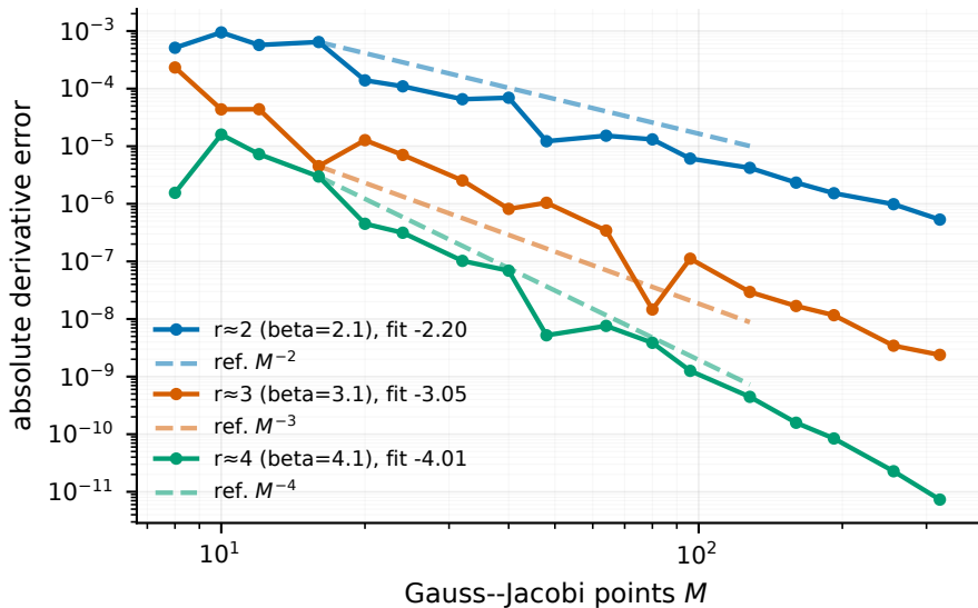
Derivative-level Type-I finite-smooth benchmark
