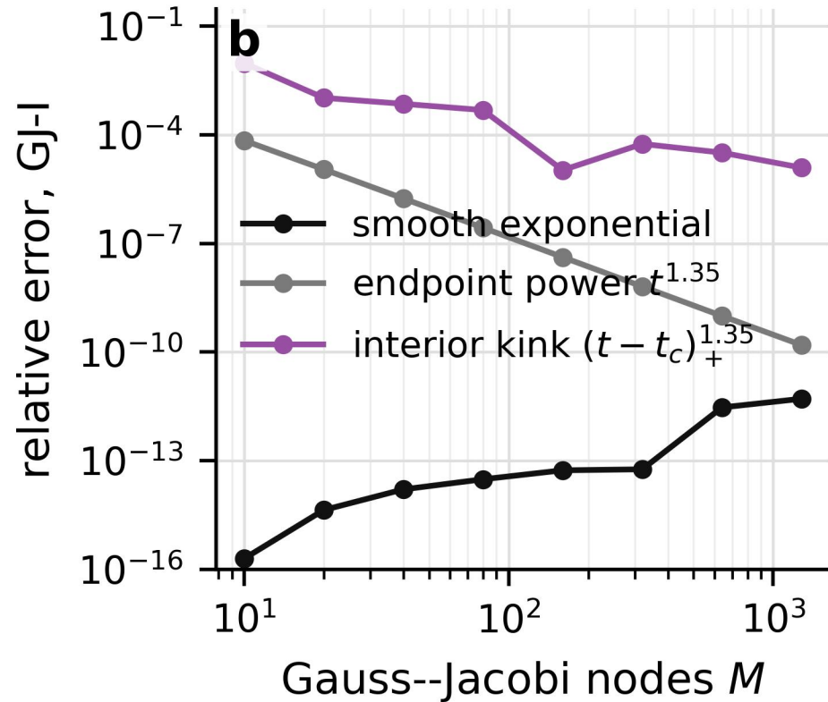
regularity controls convergence
