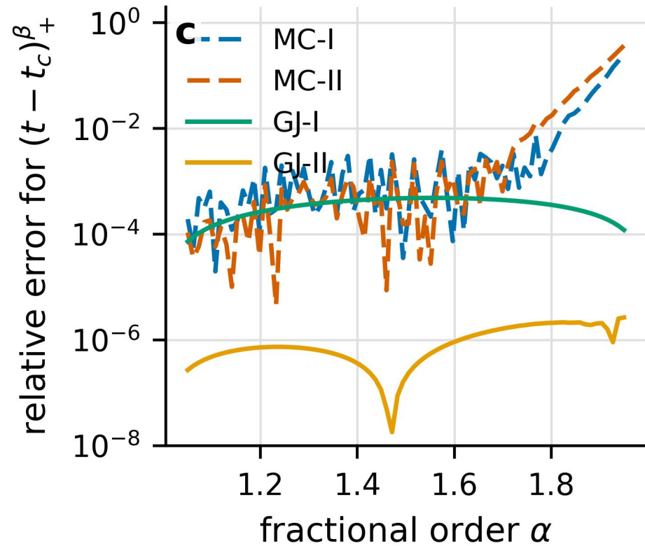
interior non-smooth point
