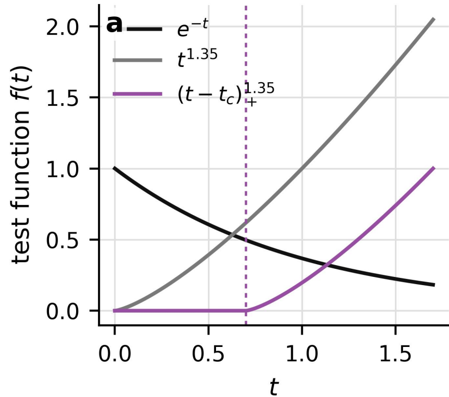
smooth vs non-smooth tests
