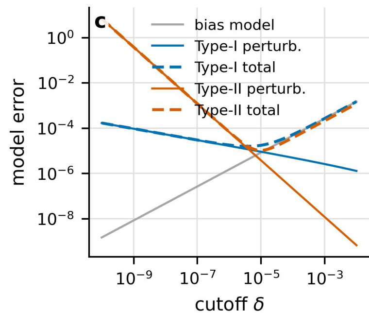
U-shaped trade-off, \alpha = 1.50
