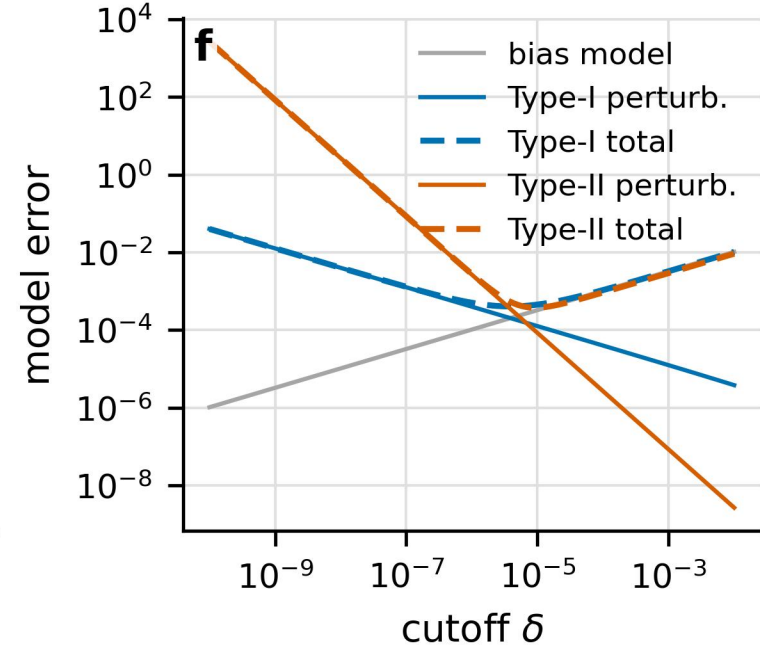
U-shaped trade-off, \alpha = 1.75
