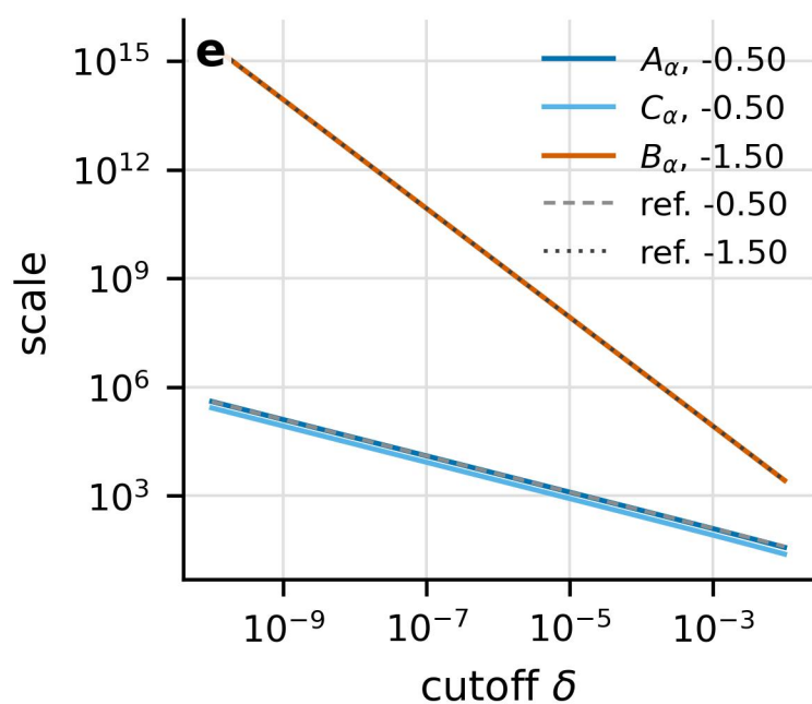
conditioning integrals, \alpha = 1.75
