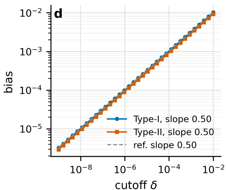
regularization bias, \alpha = 1.75
