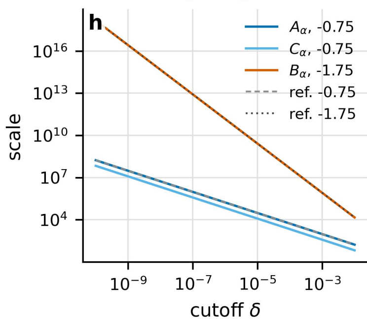
conditioning integrals, \alpha = 1.75
