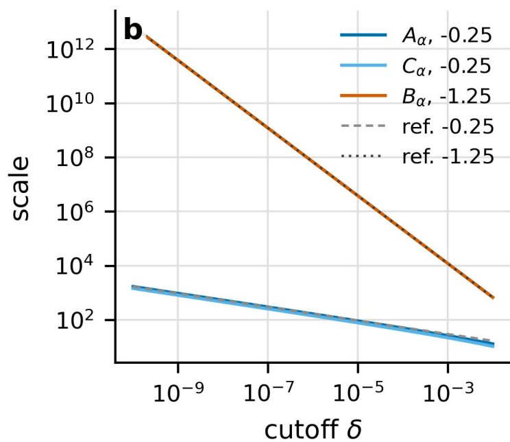
conditioning integrals, \alpha = 1.50
