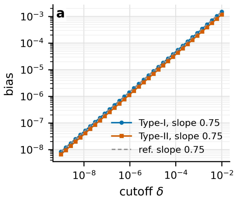
regularization bias, \alpha = 1.50
