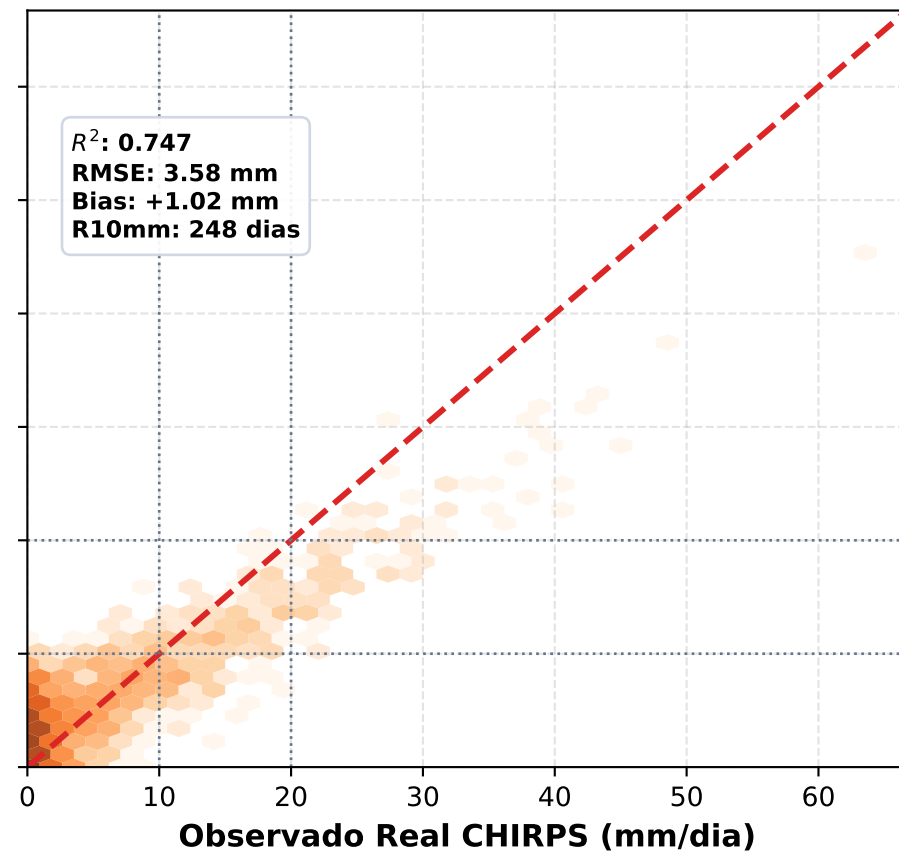
ResLSTM (2018)
