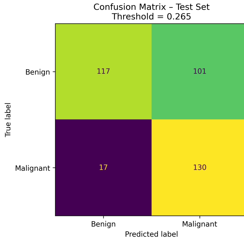
Figure 14: Confusion matrix
