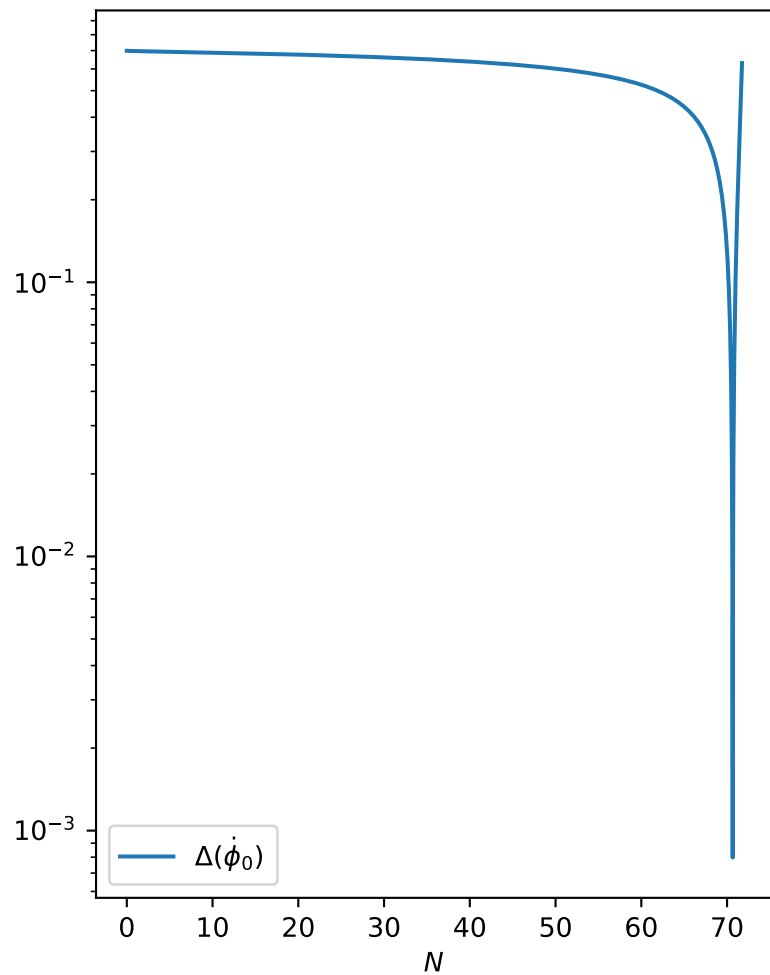
\phi_0 and \dot{\phi}_0 absolute difference
