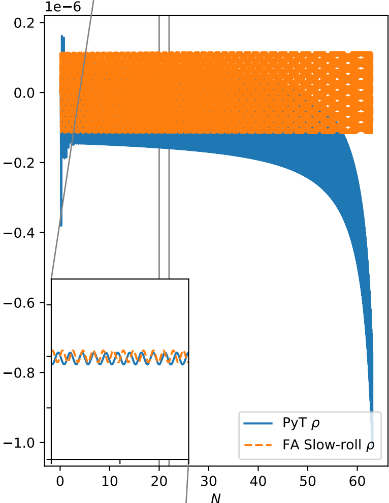
\rho and \dot{\rho} solutions
