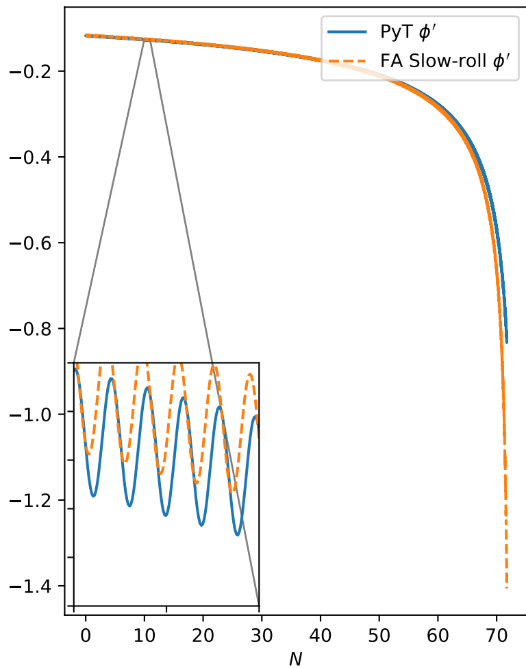
\phi and \phi' solutions
