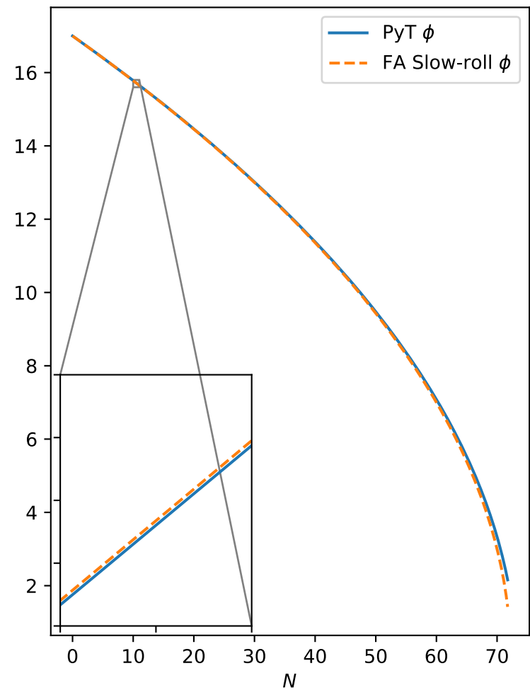
\phi and \phi' solutions
