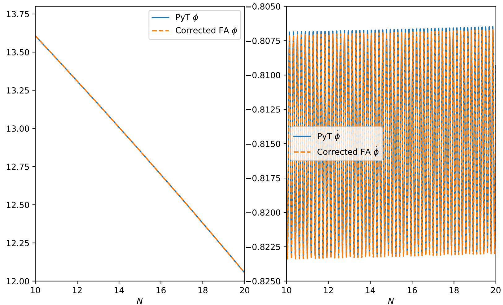
FA \phi_0 and \dot{\phi}_0 small window
