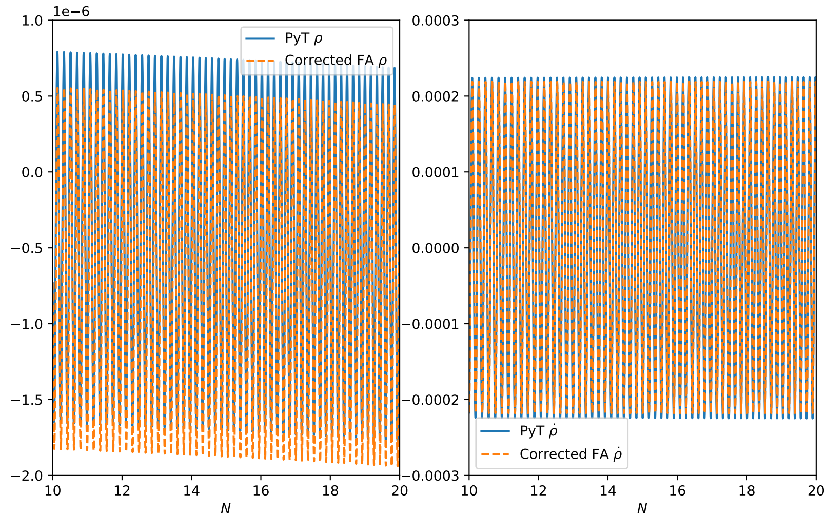
FA \rho_0 and \dot{\rho}_0 small window
