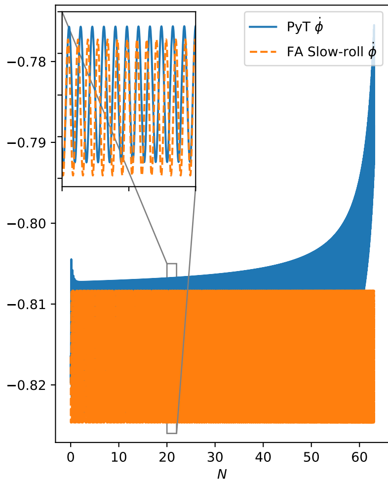
\phi and \dot{\phi} solutions
