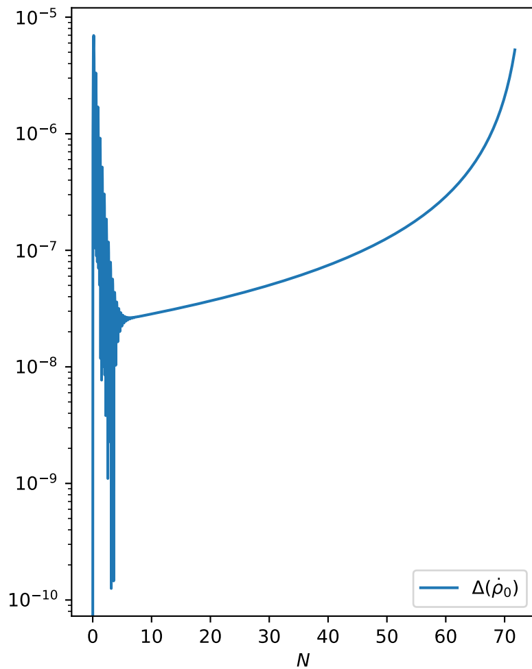
\rho_0 and \dot{\rho}_0 absolute difference
