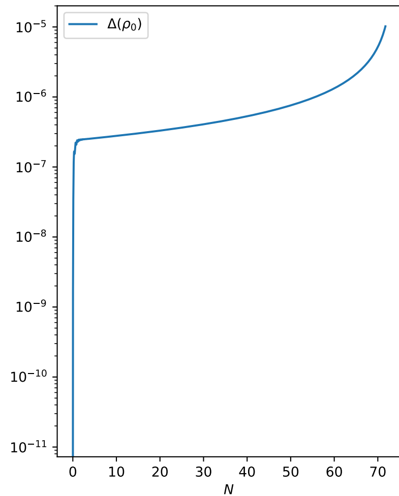
\rho_0 and \dot{\rho}_0 absolute difference
