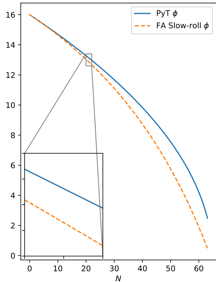
\phi and \dot{\phi} solutions
