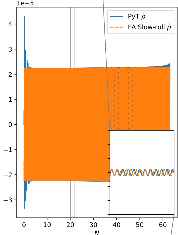
\rho and \dot{\rho} solutions
