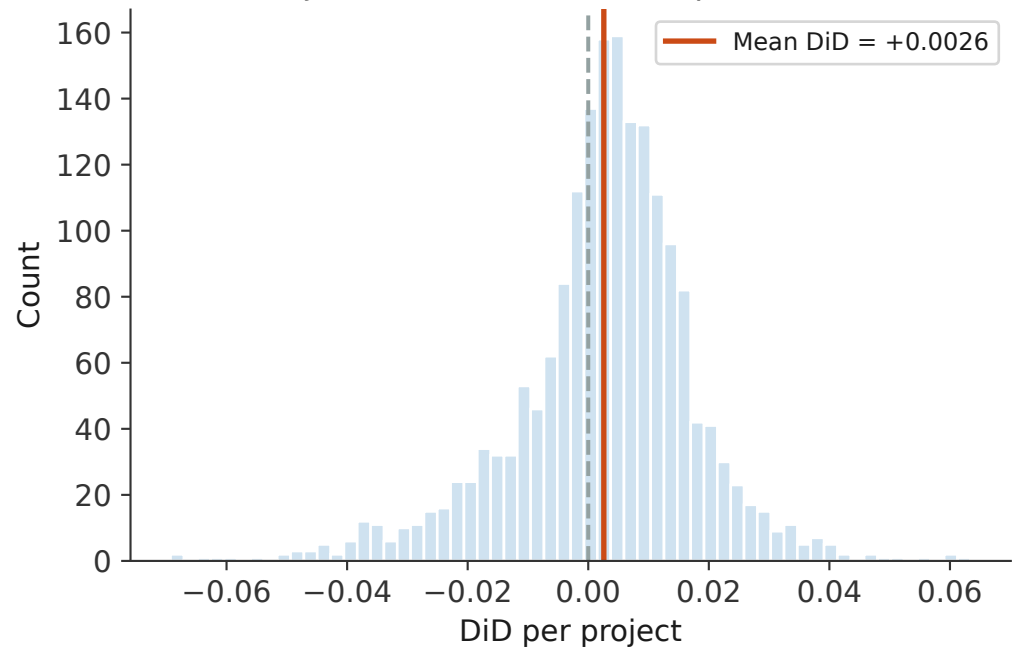
Project-level DiD ( t = 7.33 , p = 0.0000 )
