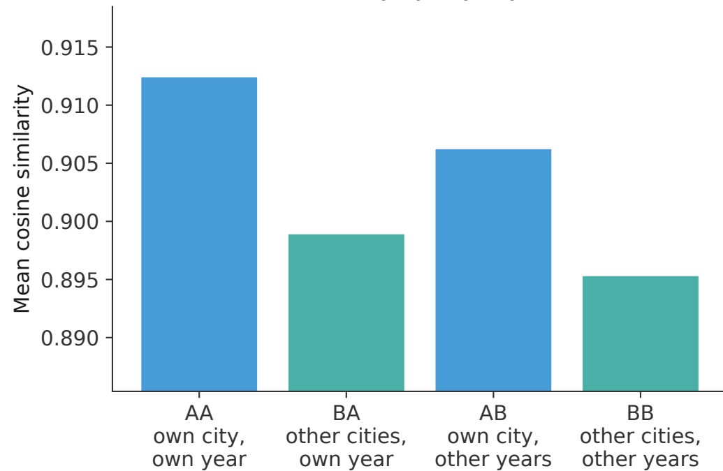
DiD: similarity by city × year cell
