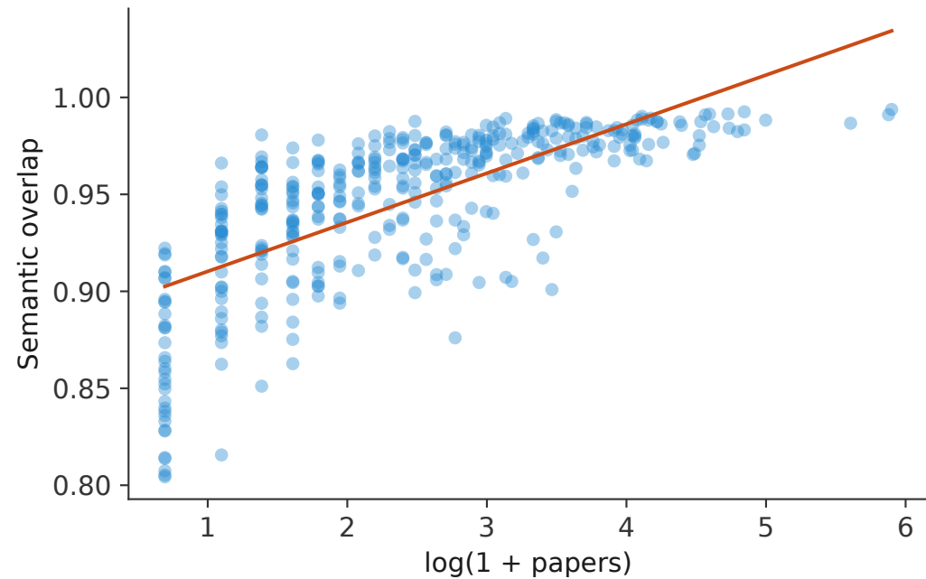
Overlap vs. city size r = 0.71 , p = 0.000
