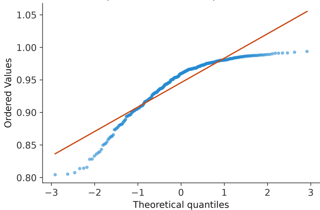
QQ plot: semantic overlap vs. normal
