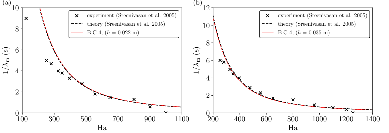
FIG. 8. Comparison of the total damping time which is the inverse of the damping rate \lambda_m = \lambda_o + \lambda_v , with experimental measurements and theoretical predictions of [13] as a function of the Hartmann number Ha at two different layer depths: a) h = 0.022\text{ m} and b) h = 0.035\text{ m} of the liquid metal. The wave mode of the free surface wave was (1, 0).
