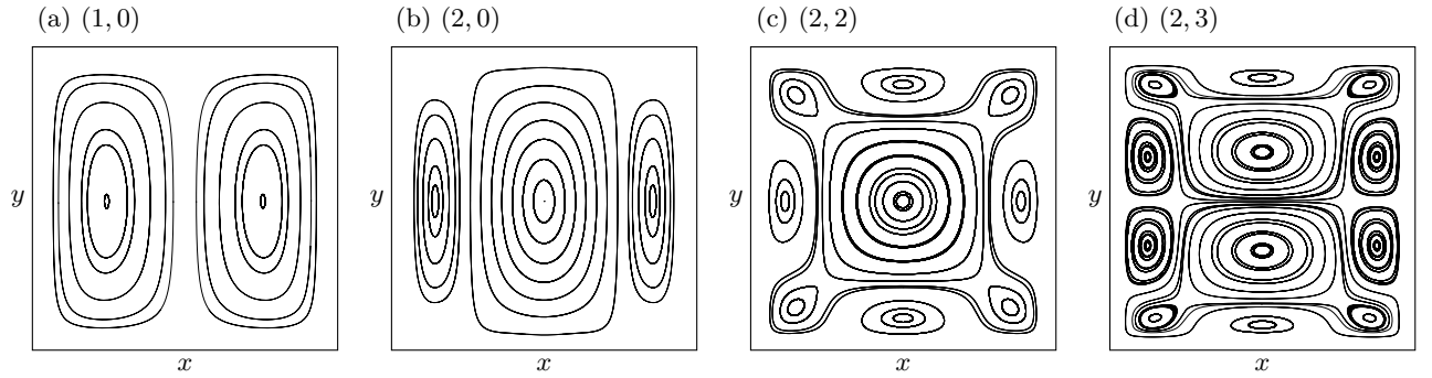
FIG. 5. More examples of induced eddy current streamlines in the horizontal x - y plane for wave modes a) (1, 0), b) (2, 0), c) (2, 2) and d) (2, 3) in a system with all insulating walls (B.C 4). The total number of induced eddy currents for a given wave mode (m, n) is observed to be equal to (m + 1)(n + 1) .
