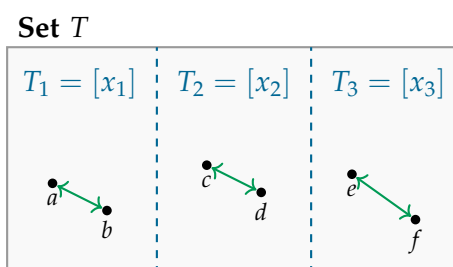
Partition of T into disjoint equivalence classes T/\equiv
