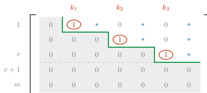
Figure 6.2: A row-reduced echelon matrix. The circled pivots are 1; everything below the green staircase is 0, and each pivot column is 0 apart from its pivot. Because k_1 < k_2 < k_3 , the pivots move strictly to the right as we descend, and the m - r zero rows are pushed to the bottom. The columns carrying a * are the ones without a pivot; they will turn into the free variables when the matrix is read back as a system.
