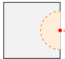
[0, 1]^2 \subseteq [0, 1]^2 ( open )
