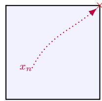
(a) [0, 1]^2 ( closed )
