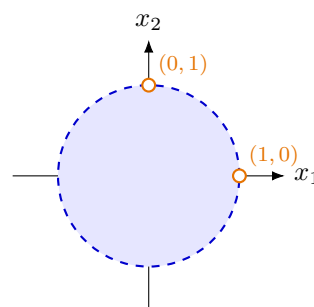
Standard metric d_2 : open disk
