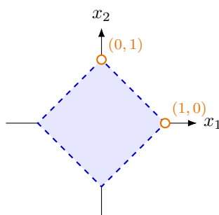
Manhattan metric d_1 : open diamond
