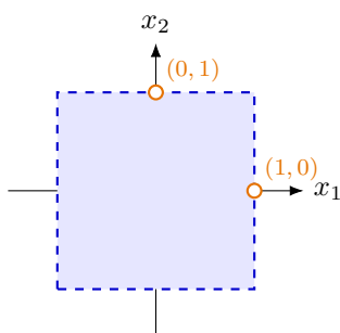
Supremum metric d_3 : open square (-1, 1)^2
