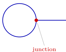
(b) lollipop
