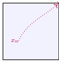
(a) [0, 1]^2 ( closed )
