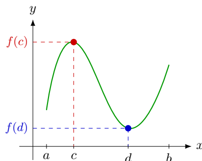
(b) on the compact K = [a, b] , f attains its maximum at c and its minimum at d
